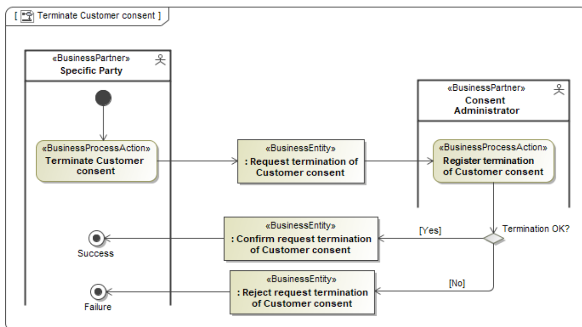
Figure 22 Business Process: Terminate Customer consent
