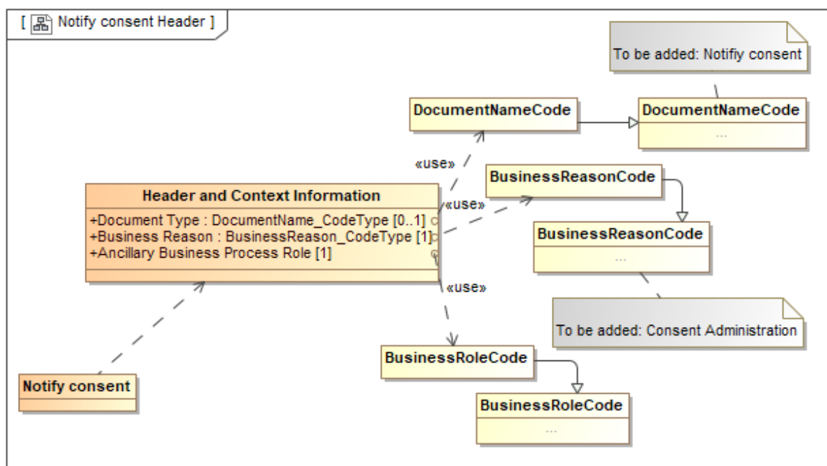
Figure 4 Class diagram: Header and Context Information Notify consent
