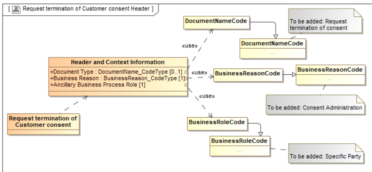
Figure 6 Class diagram: Header and Context Information Request termination of Customer consent
