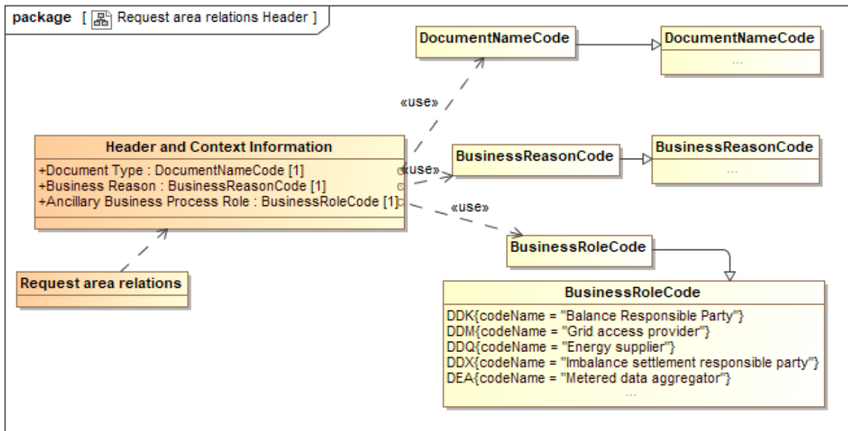
Figure 10 Class diagram: Header and Context information: Request area relations
