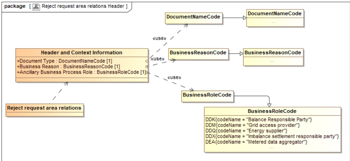
Figure 12 Class diagram: Header and Context information: Reject request area relations
