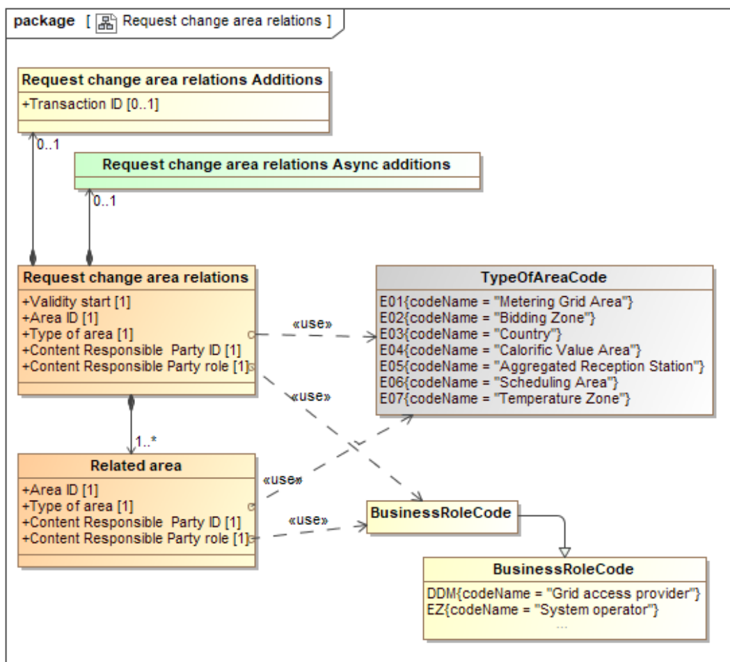
Figure 24 Class Diagram: Request change area relations
