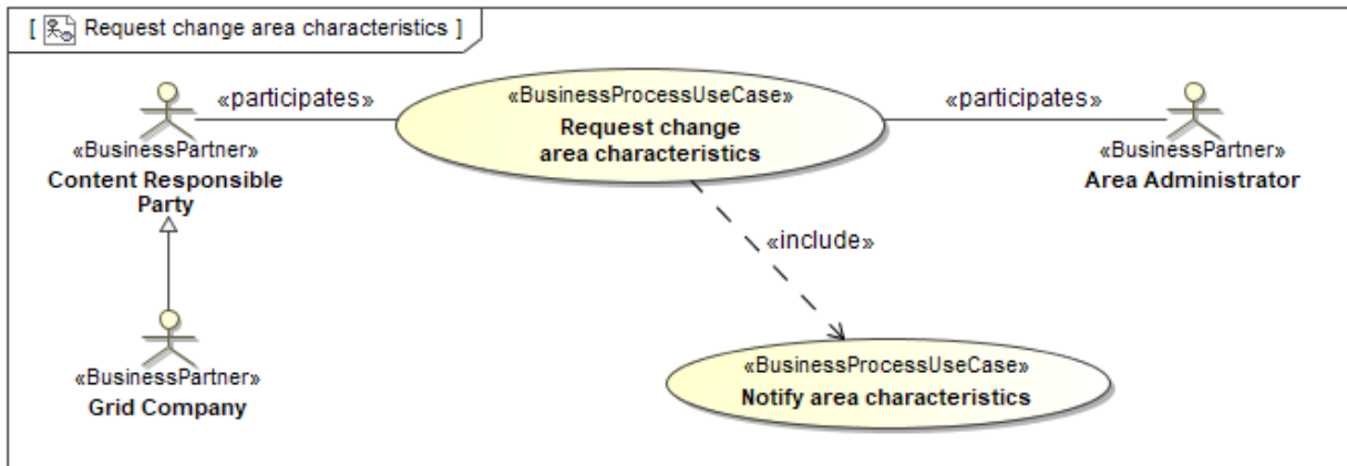
Figure 4 UseCase: Request change area characteristics
