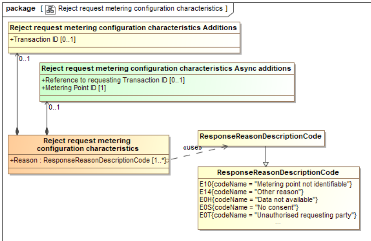
Figure 15 Reject request metering configuration characteristics
