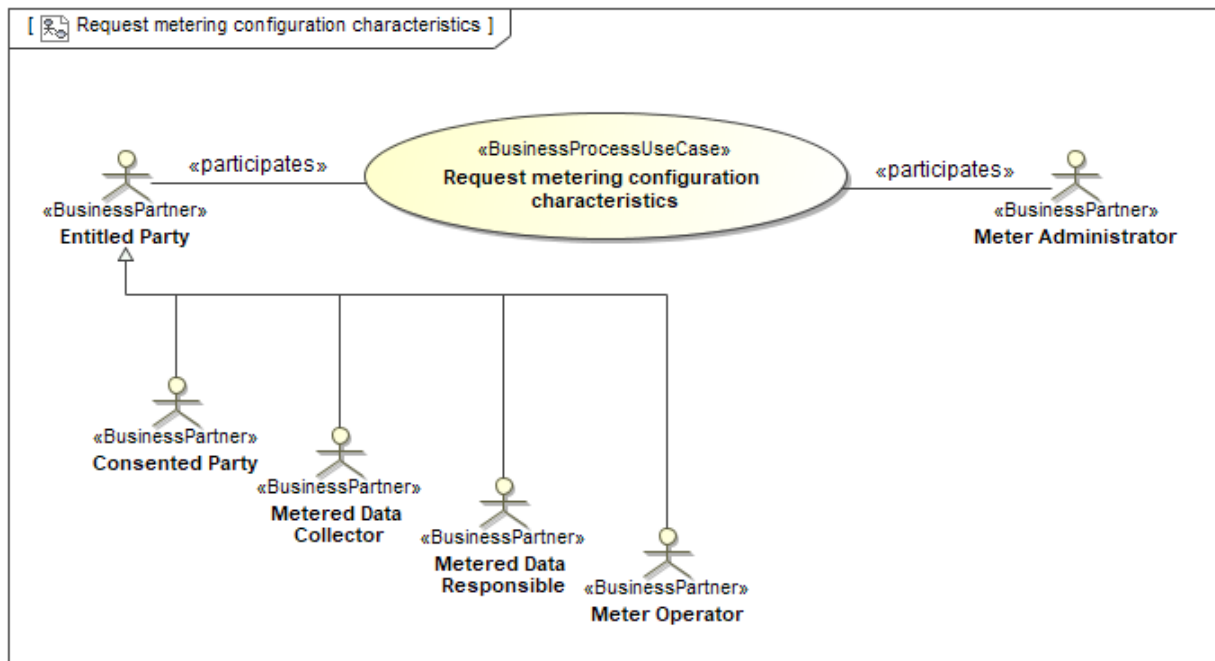
Figure 2 Request metering configuration characteristics
