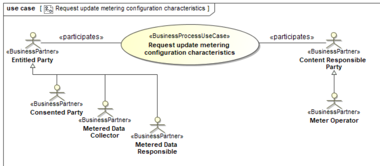
Figure 10 Request update metering configuration characteristics
