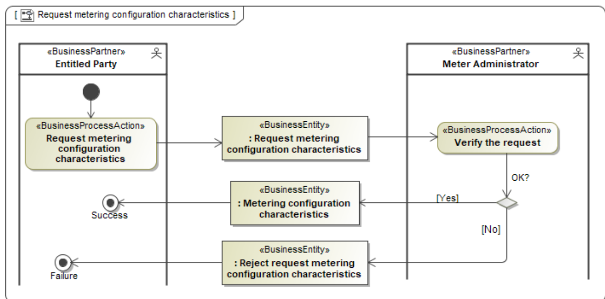
Figure 3 Business Process: Request metering configuration characteristics
