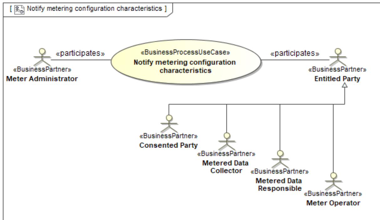
Figure 8 Notify metering configuration characteristics
