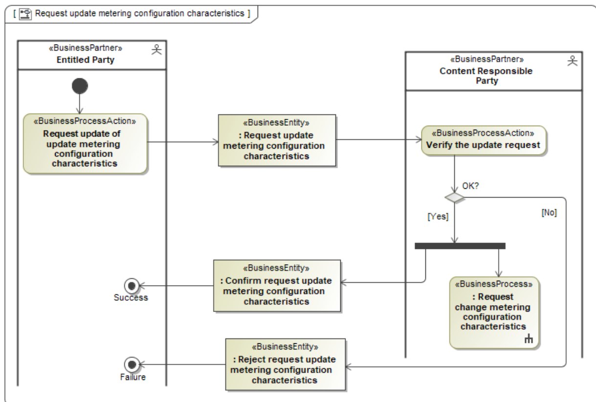
Figure 11 Business Process: Request update metering configuration characteristics
