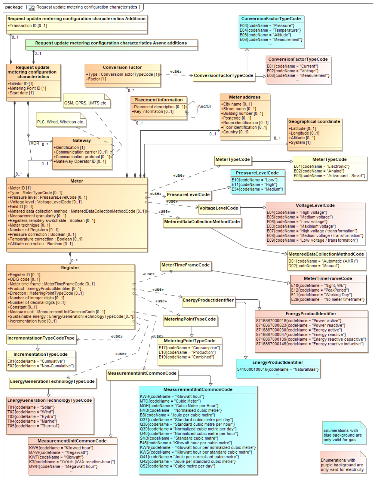
Figure 19 Request update metering configuration characteristics
