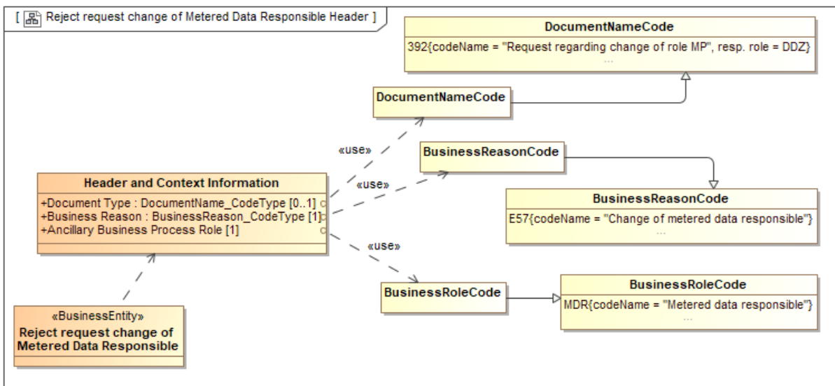
Figure 14 Class diagram: Header and context Information Reject request change of Metered Data Responsible
