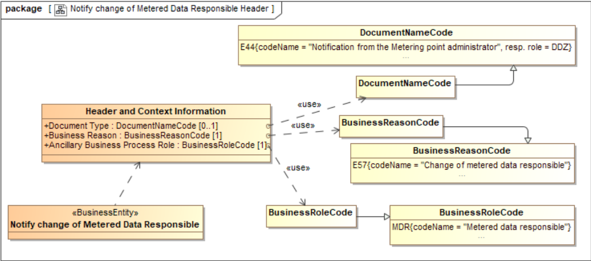
Figure 15 Class diagram: Header and context Information: Notify change of Metered Data Responsible
