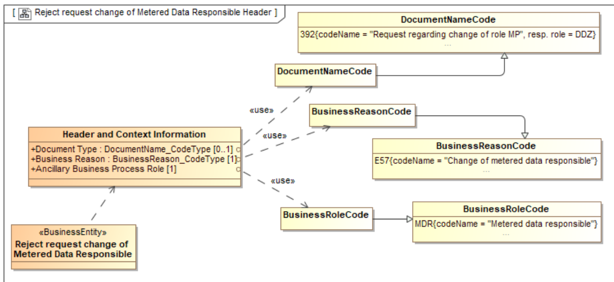
Figure 14 Class diagram: Header and context Information Reject request change of Metered Data Responsible
