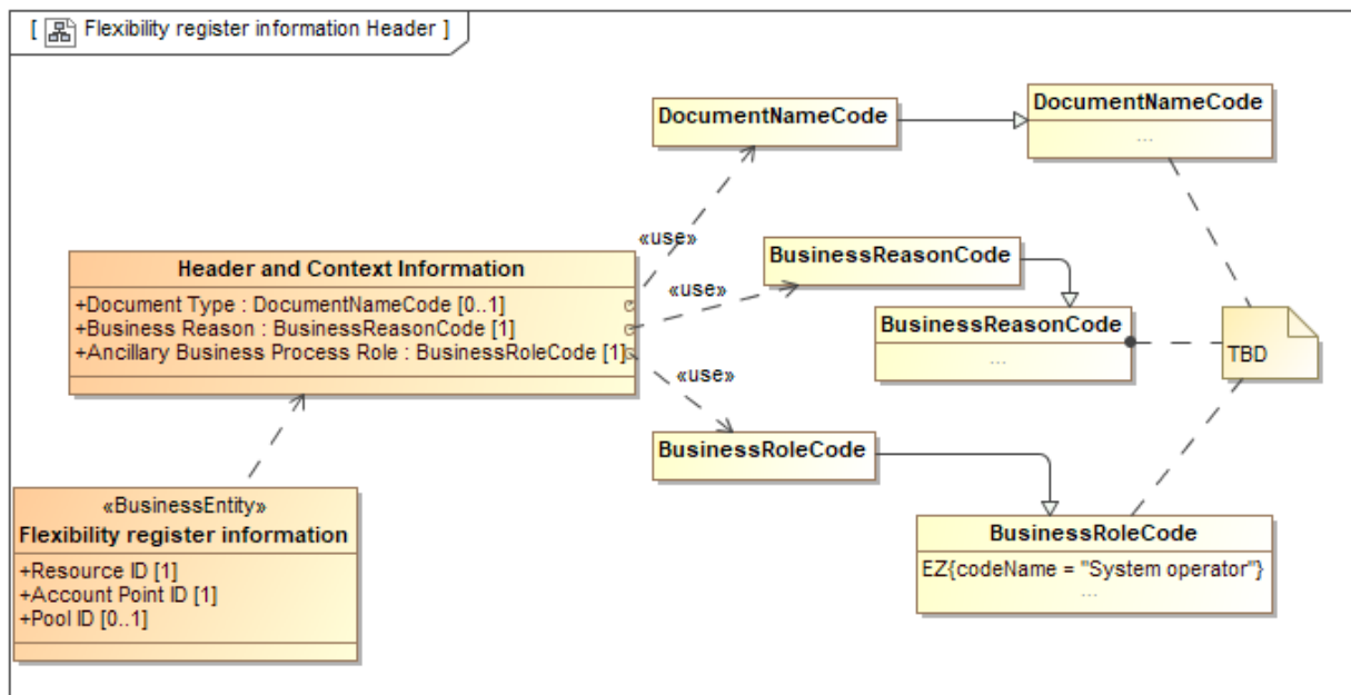
Figure 47 Class diagram: Header and Context information for Flexibility register information
