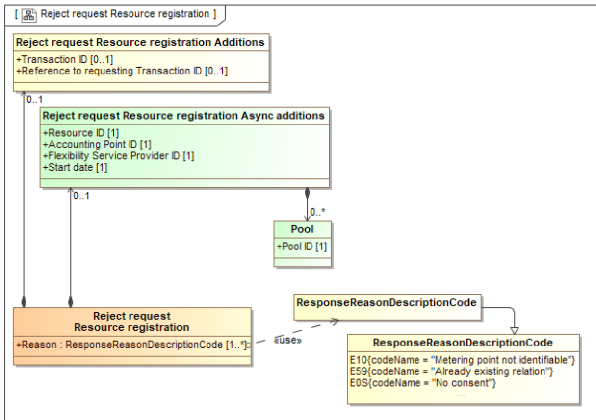
Figure 32 Class diagram: Reject request Resource registration
