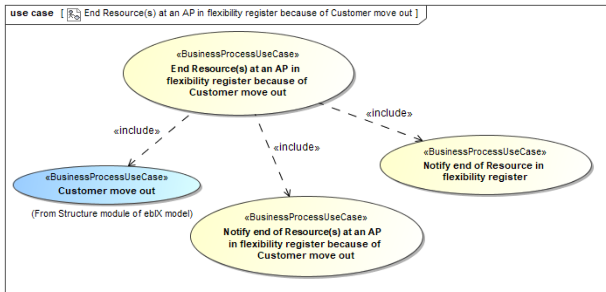
Figure 14 Business Process UseCase: End Resource(s) (AP) in flexibility register because of Customer move out
