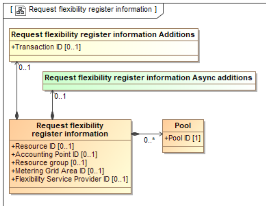
Figure 42 Class diagram: Request flexibility register information
