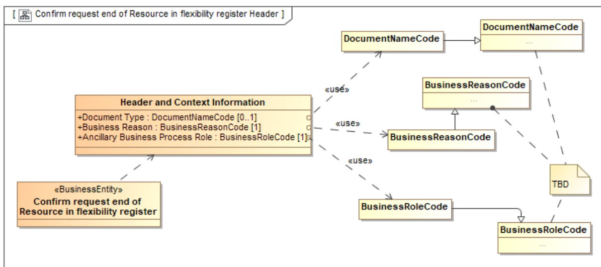
Figure 52 Class diagram: Header and Context information for Confirm request end of Resource in flexibility register
