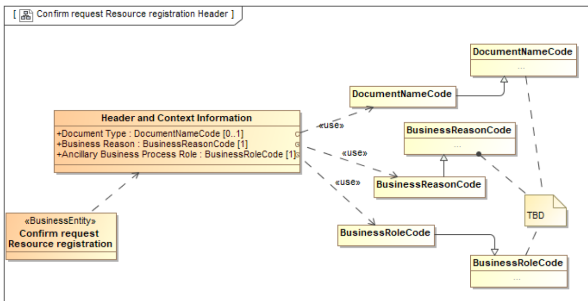
Figure 45 Class diagram: Header and Context information for Confirm request Resource registration
