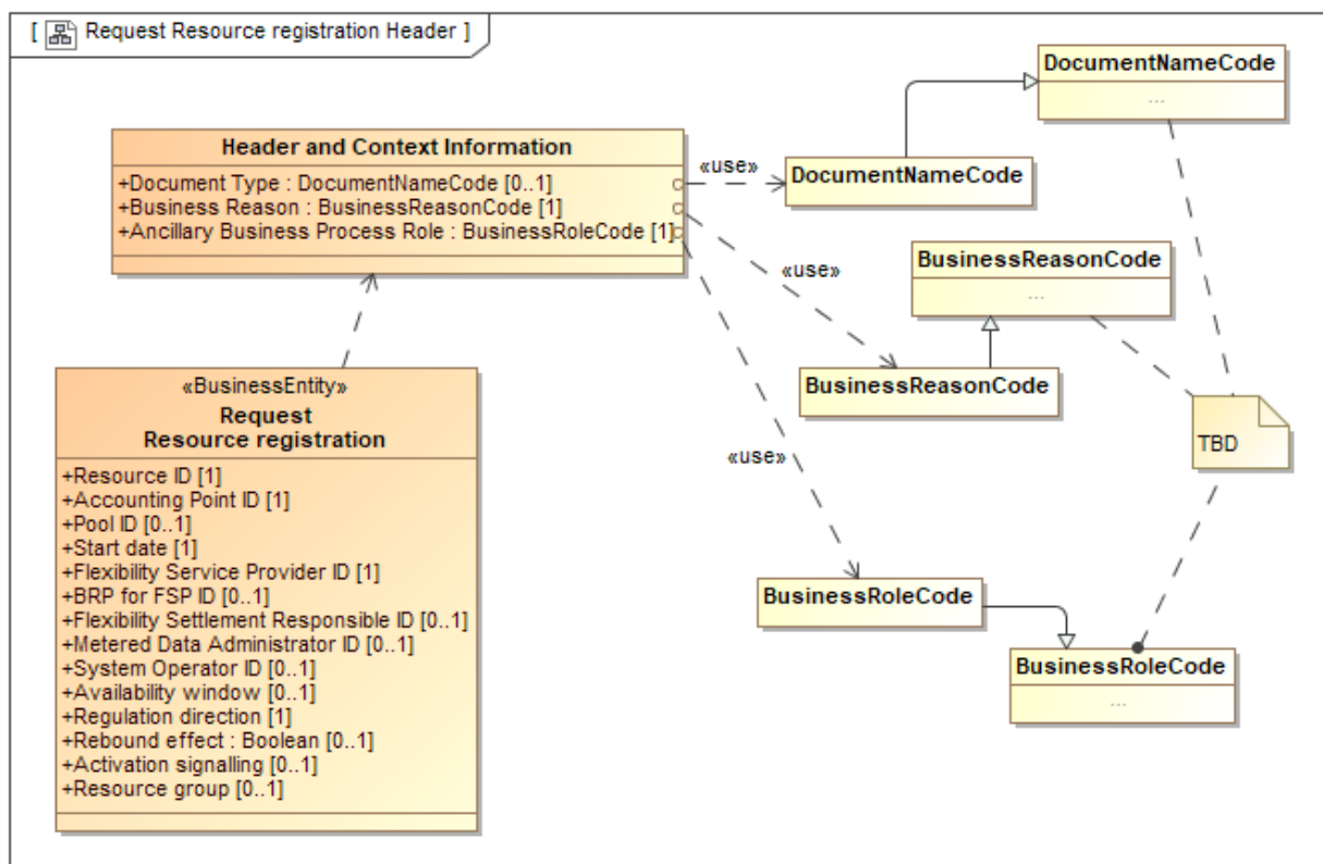
Figure 44 Class diagram: Header and Context information for Request Resource registration
