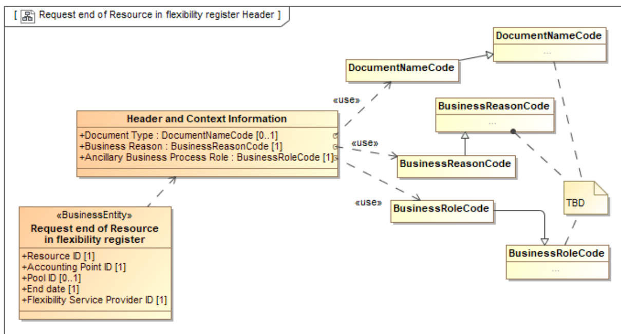
Figure 51 Class diagram: Header and Context information for Request end of Resource in flexibility register
