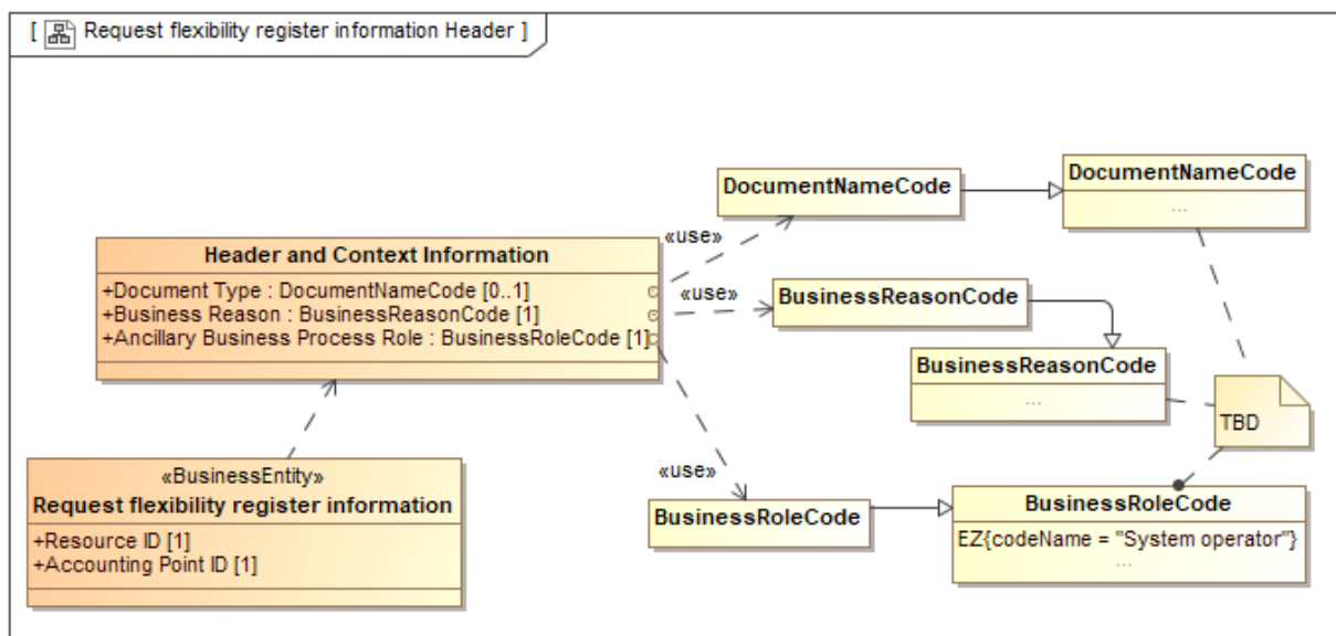
Figure 56 Class diagram: Header and Context information for Request flexibility register information
