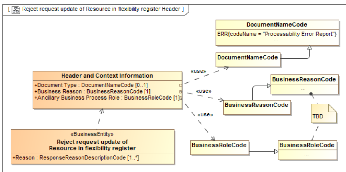
Figure 50 Class diagram: Header and Context information for Reject request update of Resource in flexibility register
