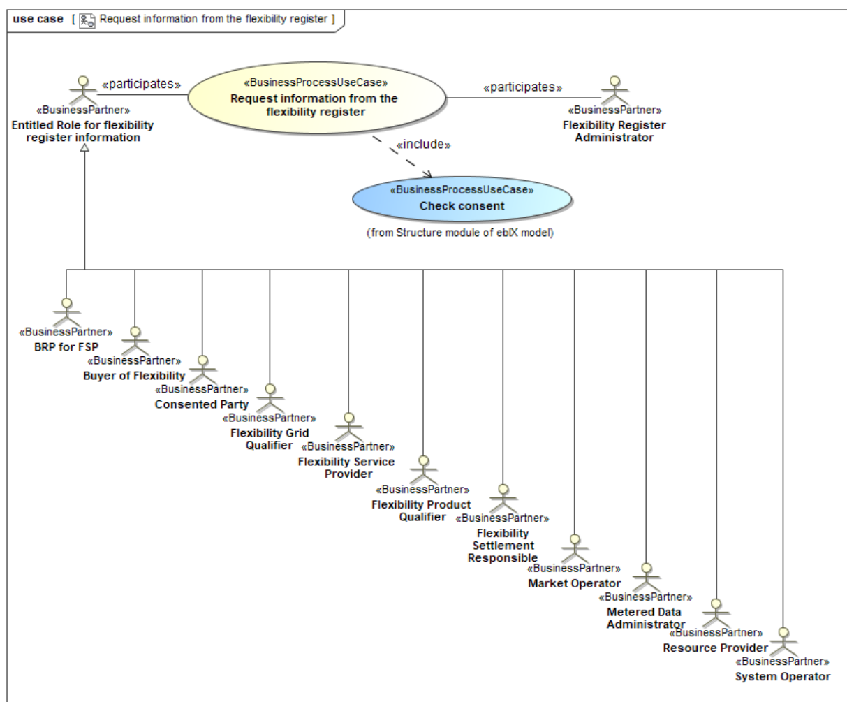
Figure 25 Business Process UseCase: Request information from the flexibility register
