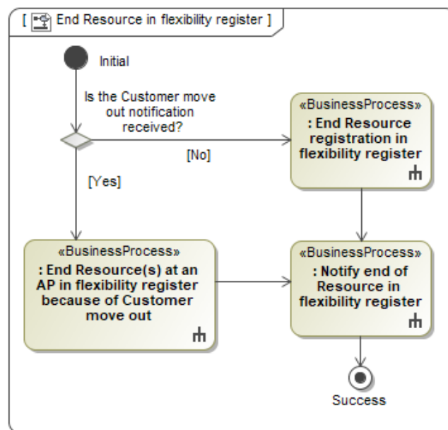
Figure 13 Business Process: End Resource in Flexibility register
