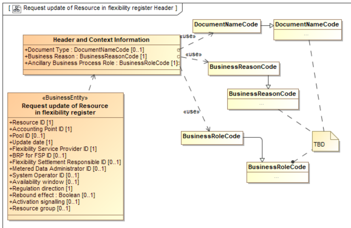
Figure 48 Class diagram: Header and Context information for Request update of Resource in flexibility register
