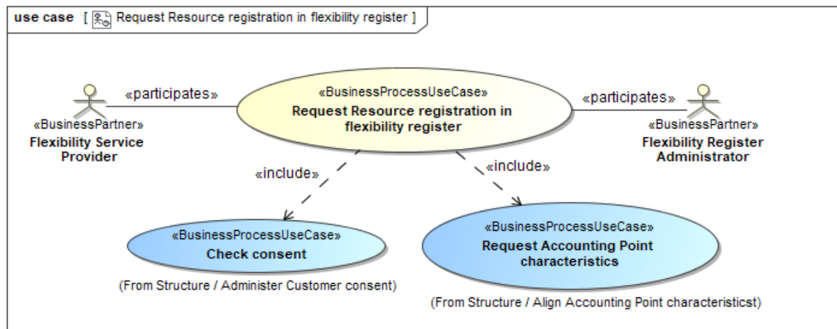
Figure 6 Business Process UseCase: Request Resource registration in flexibility register
