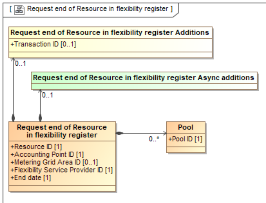
Figure 37 Class diagram: Request end of Resource in flexibility register
