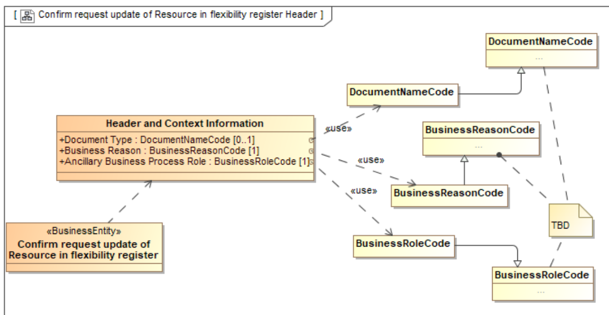
Figure 49 Class diagram: Header and Context information for Confirm request update of Resource in flexibility register
