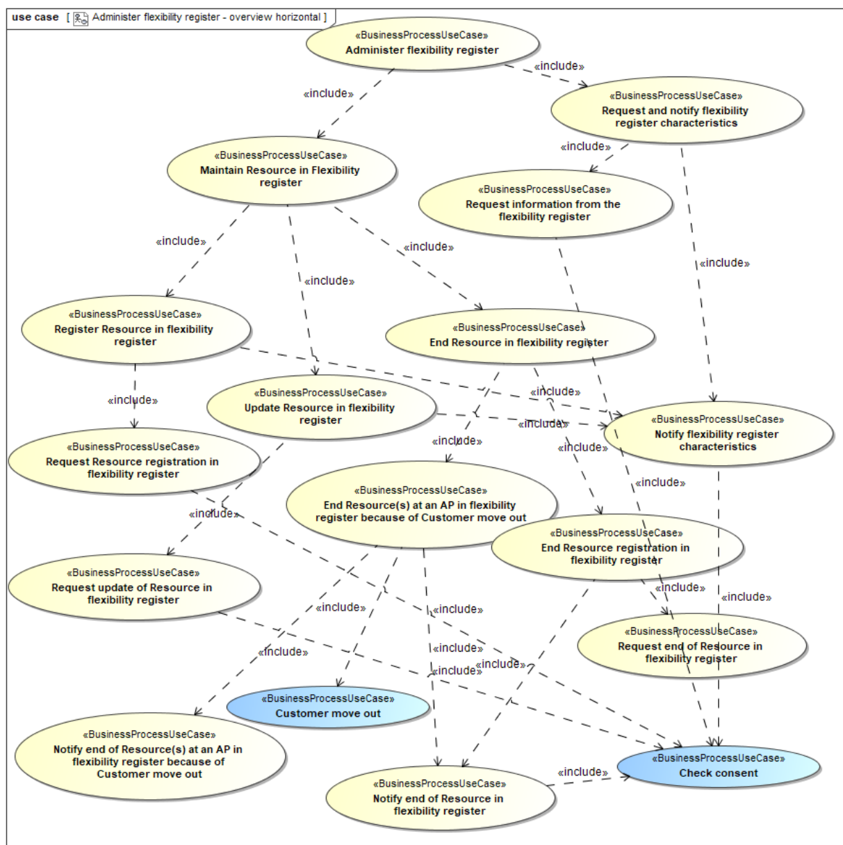
Figure 1: Overview of UseCases elaborated in this BRS for Flexibility register administration
