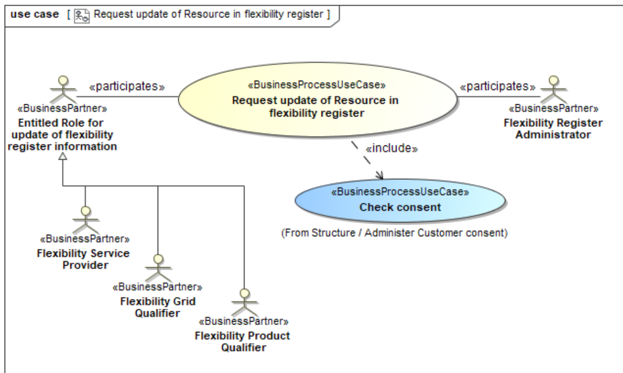
Figure 10 Business Process UseCase: Request update Resource in flexibility register
