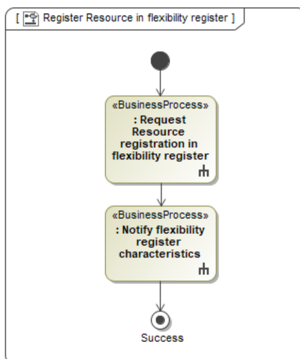
Figure 5 Business Process: Register Resource in Flexibility register
