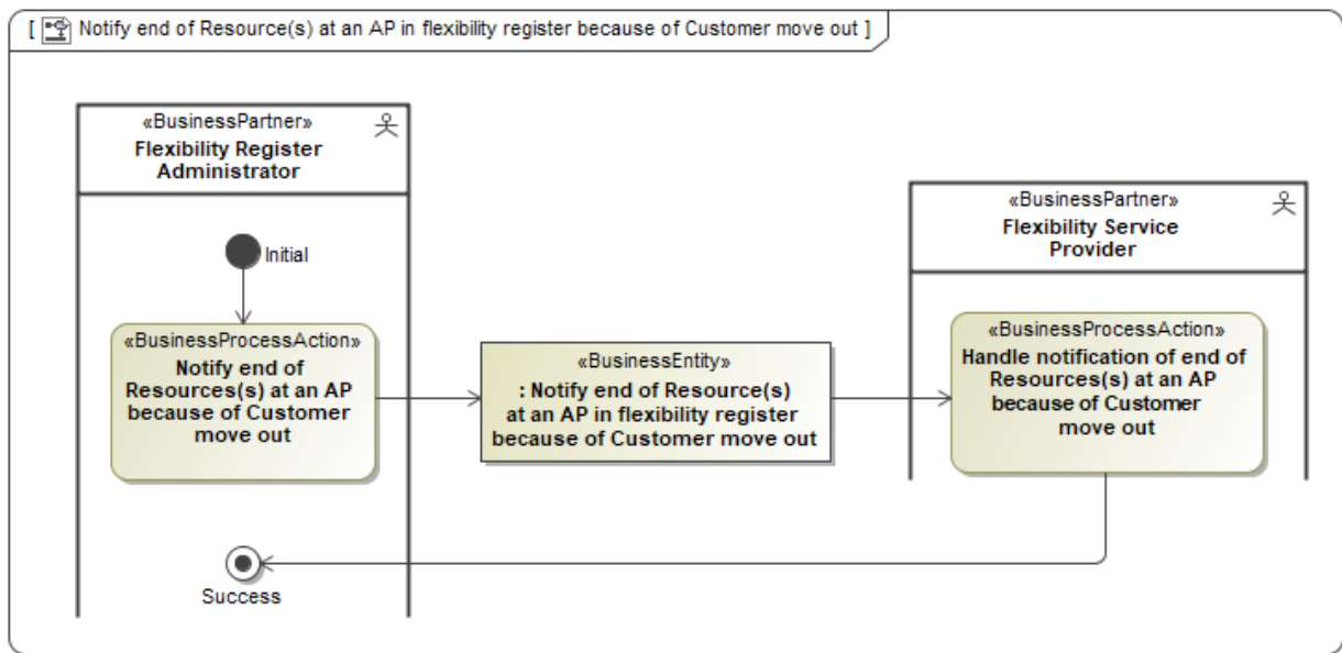
Figure 17 Business Process: Notify end of Resource(s) in flexibility register because of Customer move out
