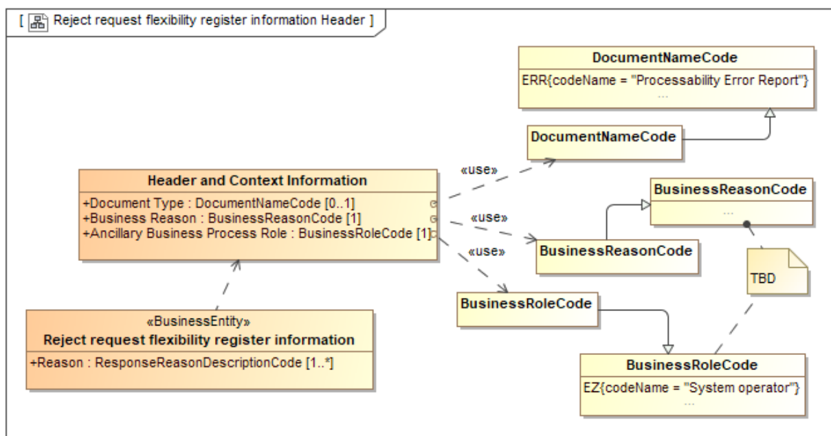
Figure 57 Class diagram: Header and Context information for Reject request flexibility register information
