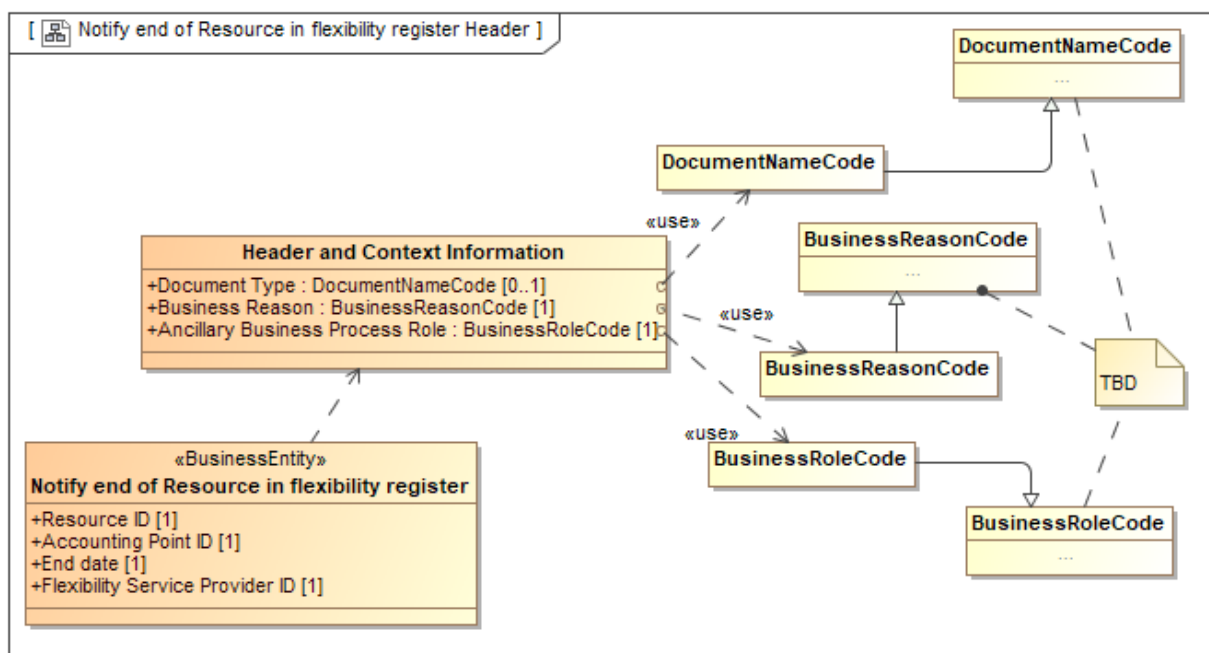
Figure 55 Class diagram: Header and Context information for Notify end of Resource in flexibility register
