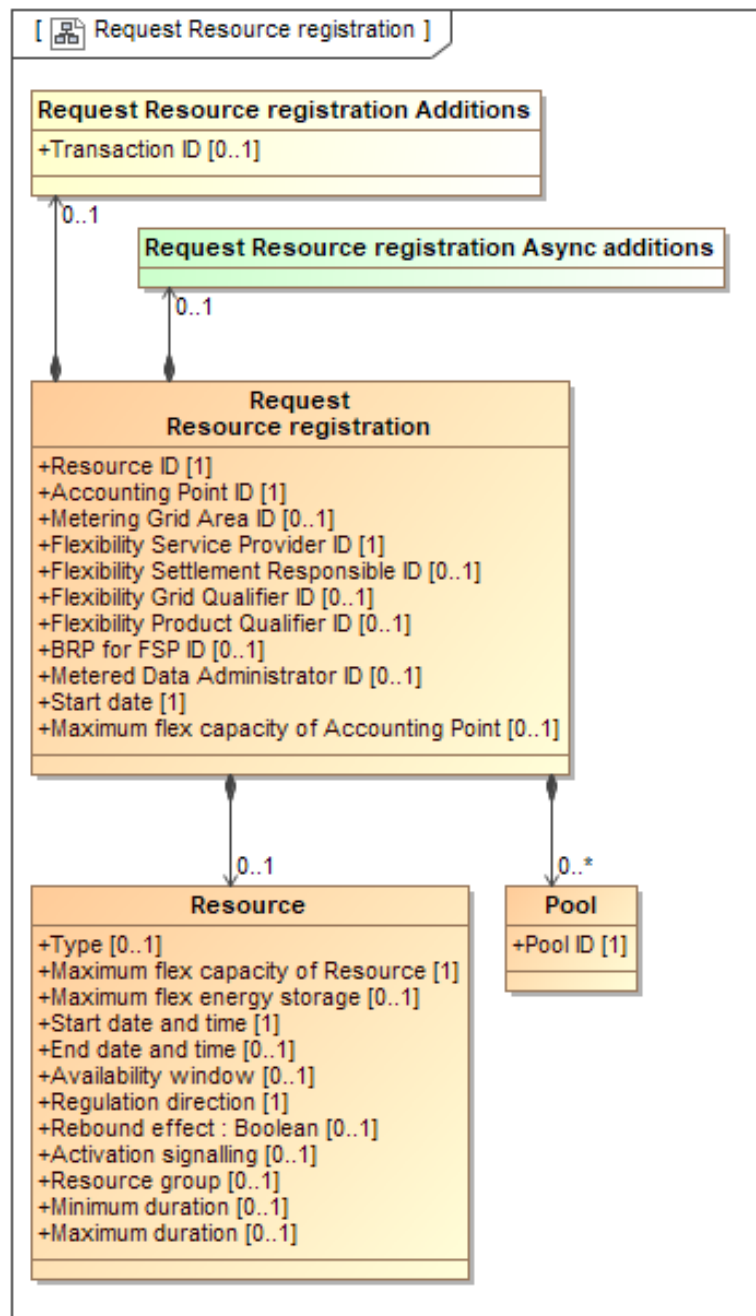
Figure 30 Class diagram: Request Resource registration
