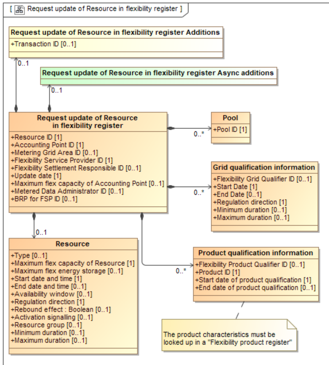
Figure 34 Class diagram: Request update of Resource in flexibility register
