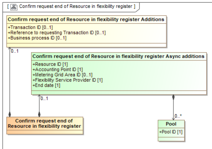
Figure 38 Class diagram: Confirm request end of Resource in flexibility register
