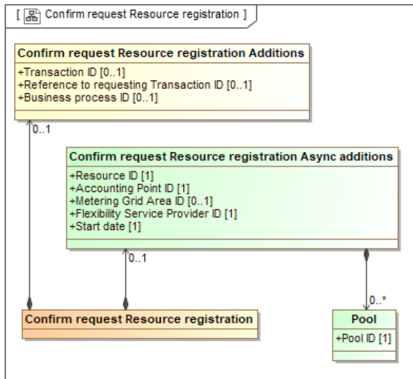
Figure 31 Class diagram: Confirm request Resource registration
