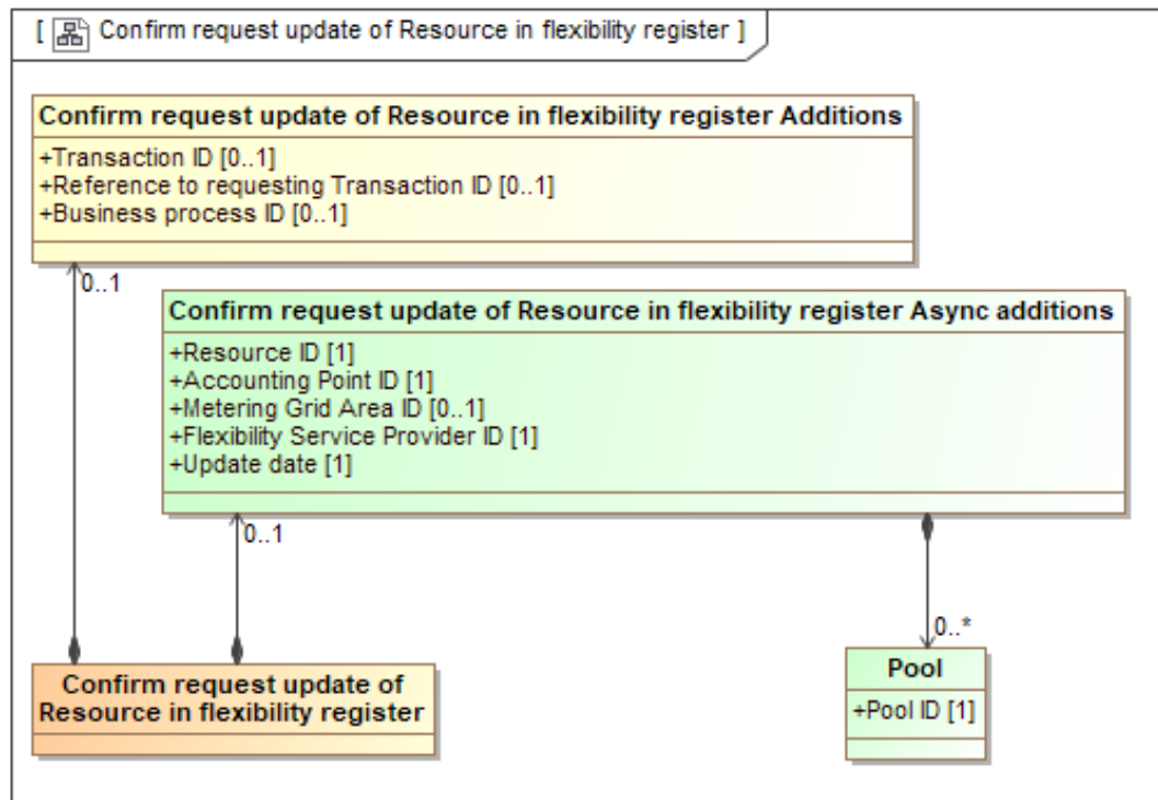
Figure 35 Class diagram: Confirm request update of Resource registration in flexibility register
