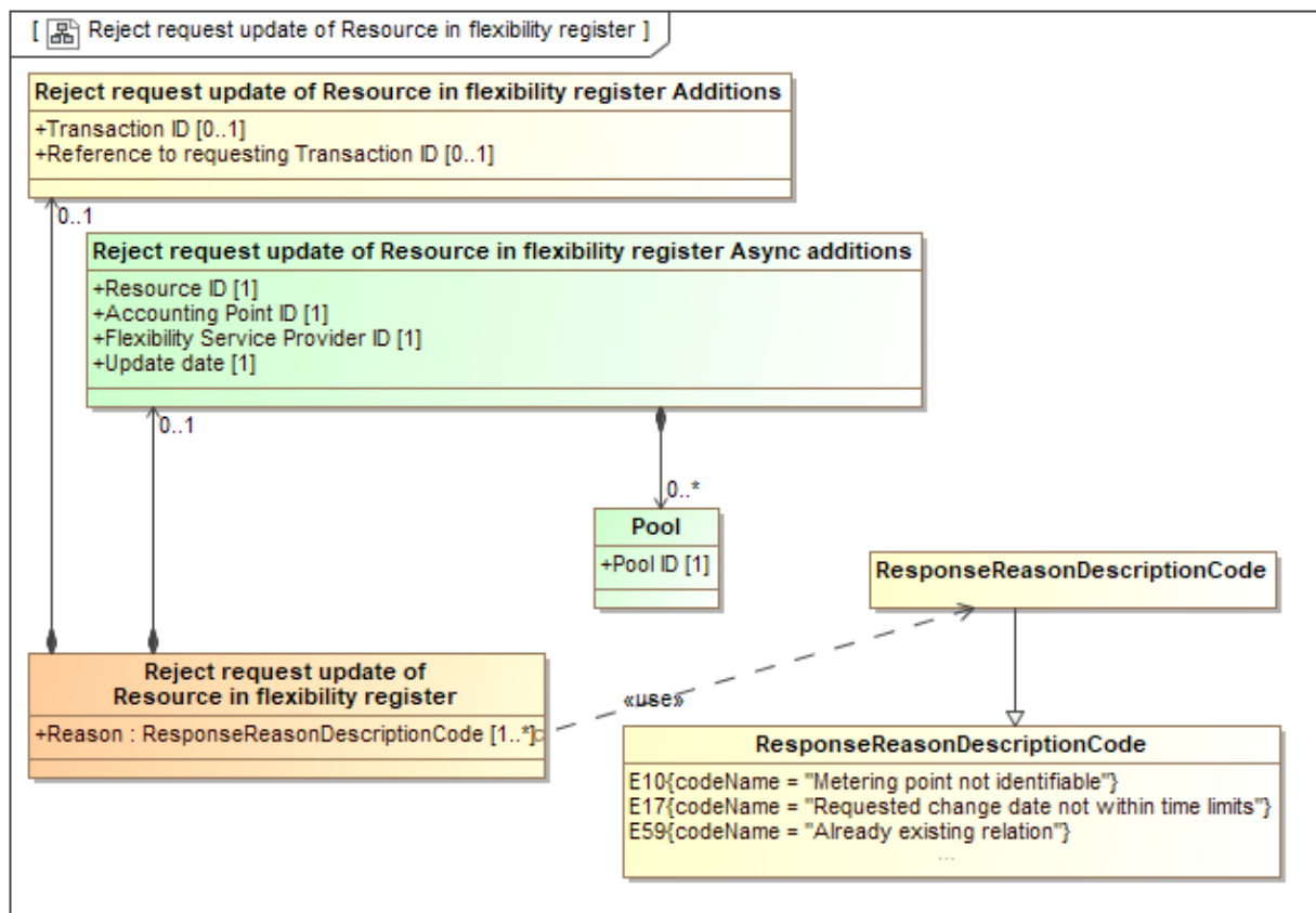
Figure 36 Class diagram: Reject request update of Resource in flexibility register
