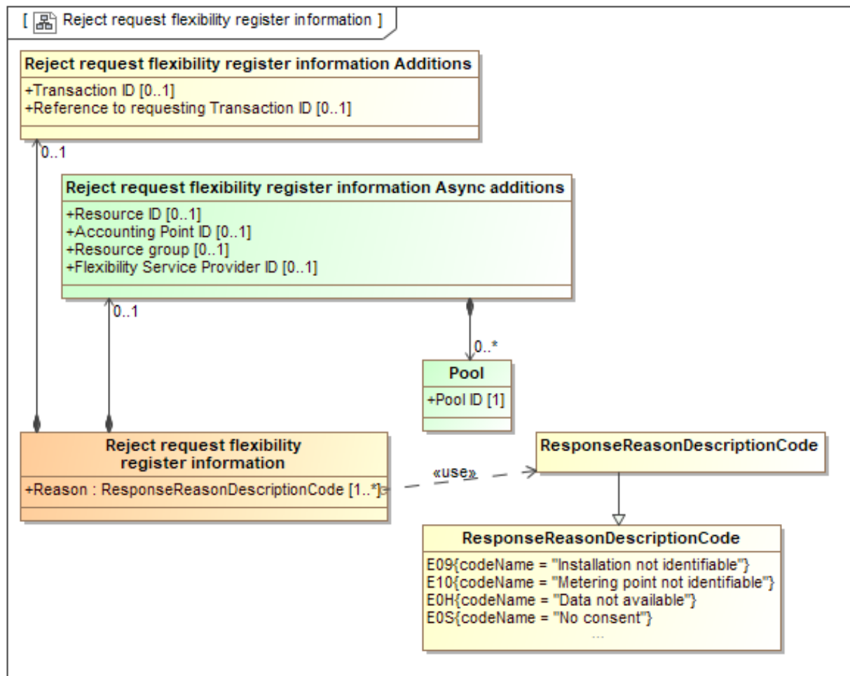
Figure 43 Class diagram: Reject request flexibility register information
