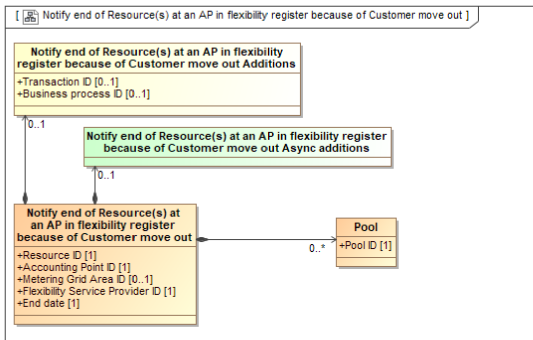
Figure 40 Class diagram: Notify end of Resource(s) at an Accounting Point in flexibility register because of Customer move out
