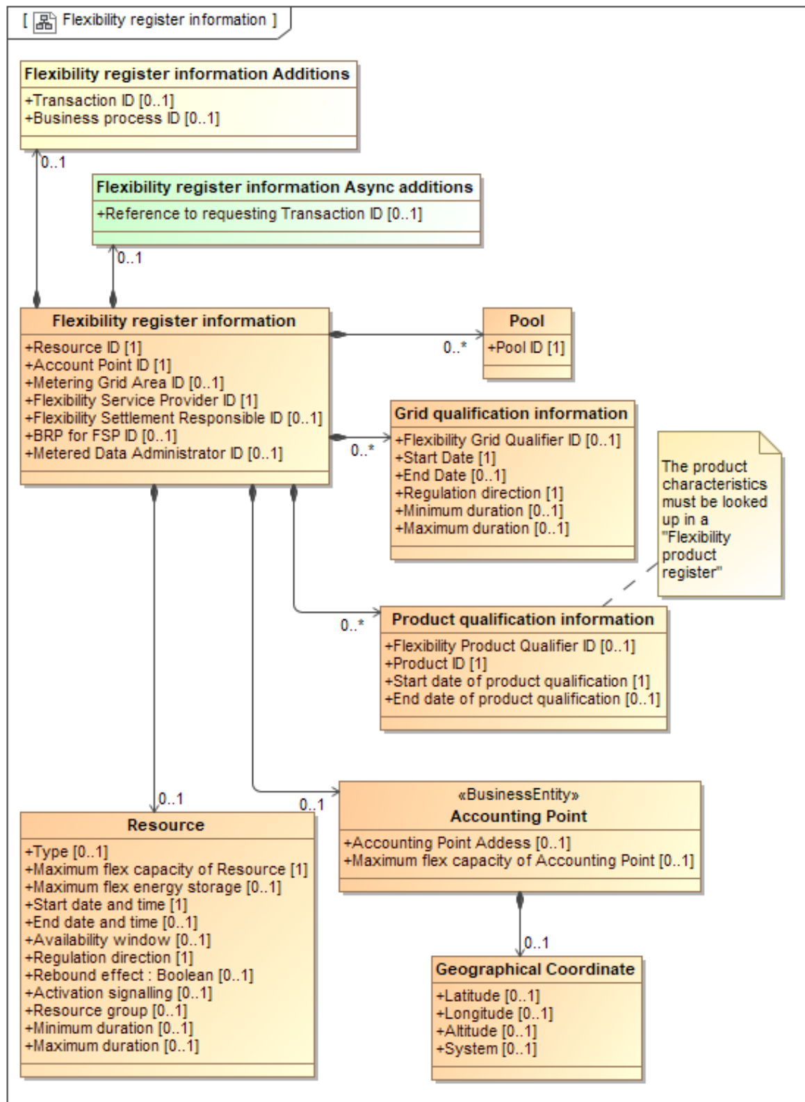
Figure 33 Class diagram: Flexibility register information
