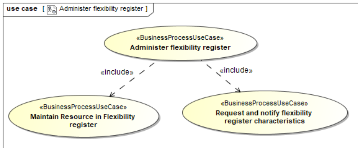
Figure 2 Business Process UseCase: Flexibility register administration
