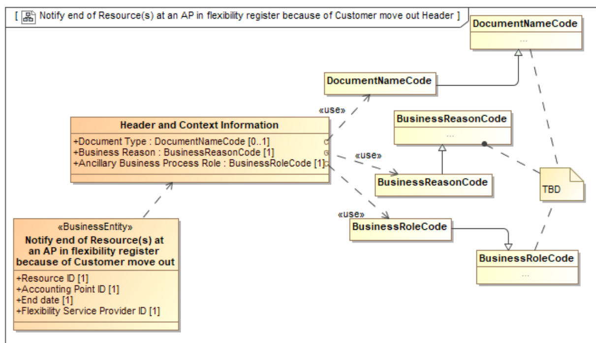
Figure 54 Class diagram: Header and Context information for Notify end of Resource(s) at an AP in flexibility register because of Customer move out
