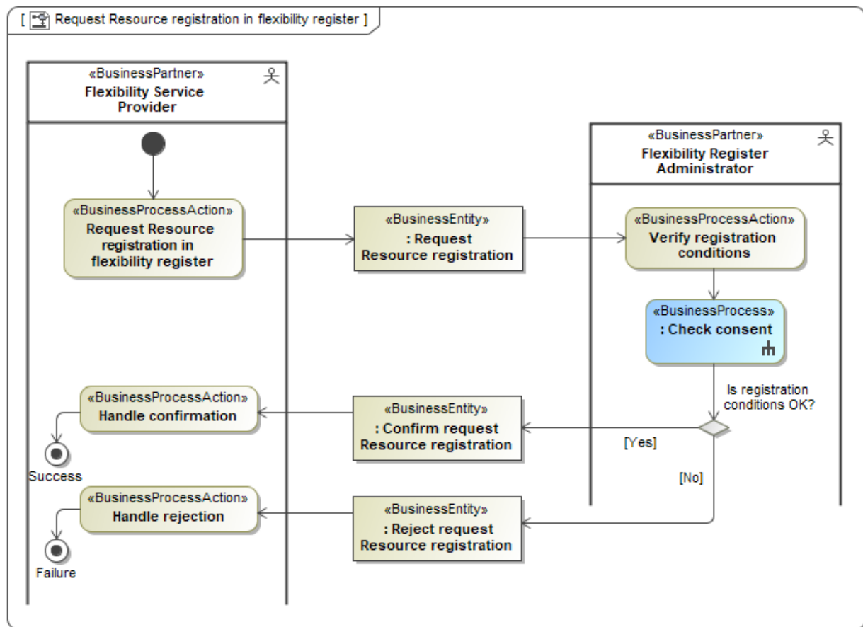
Figure 7 Business Process: Request Resource registration in flexibility register
