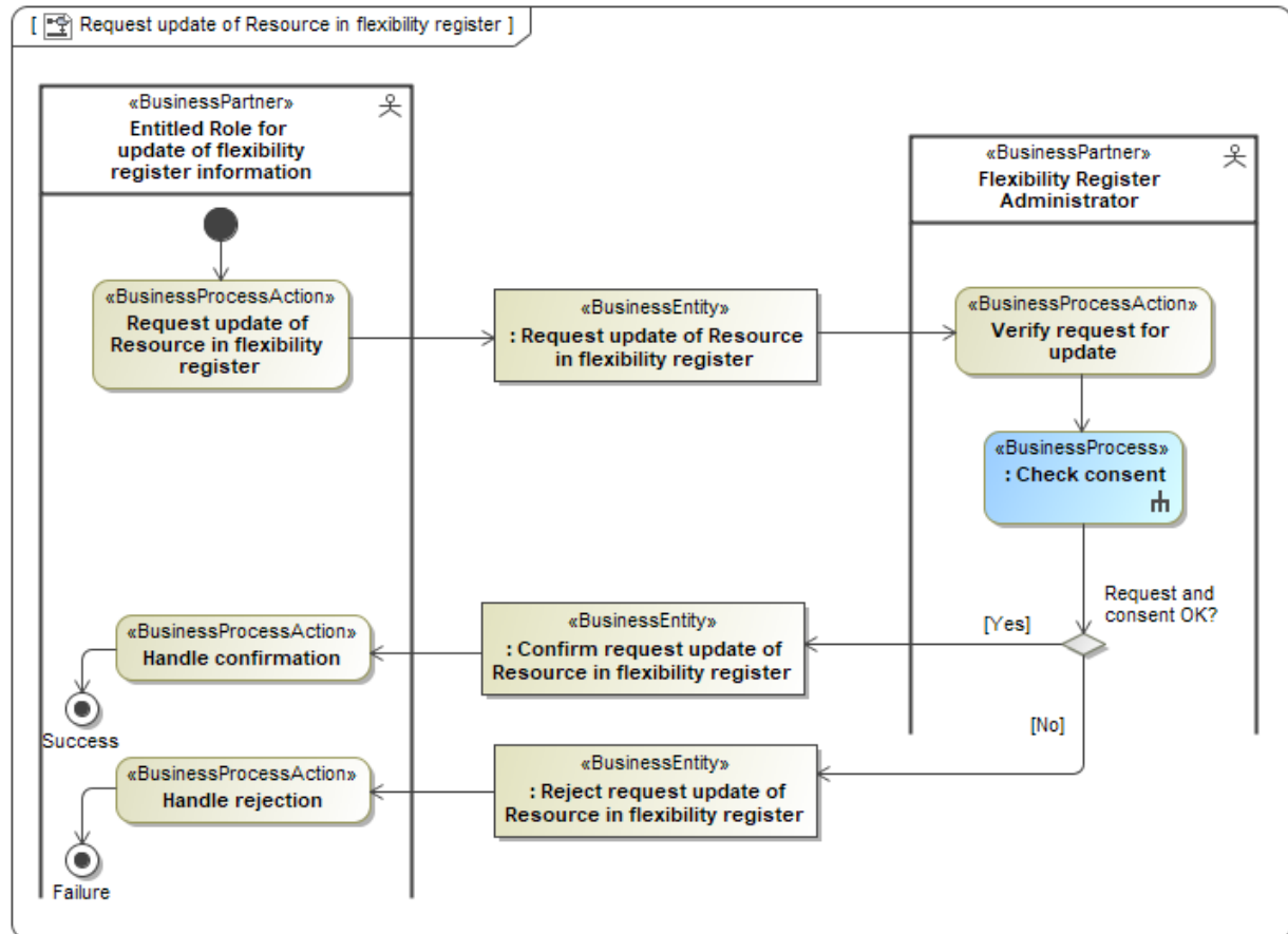
Figure 11 Business Process: Request update Resource in flexibility register
