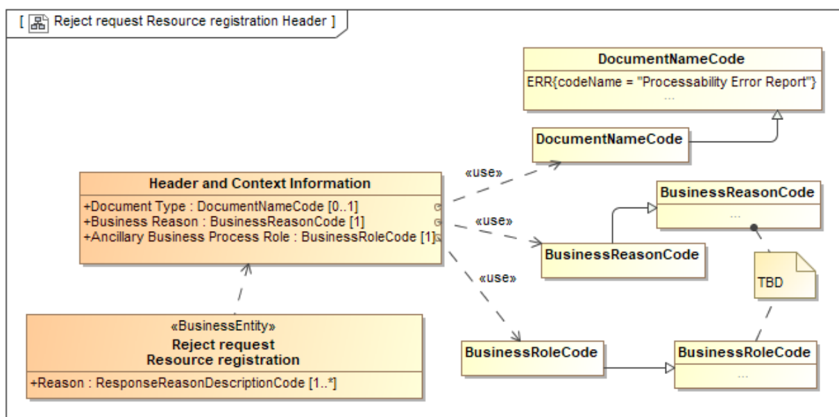
Figure 46 Class diagram: Header and Context information for Reject request Resource registration
