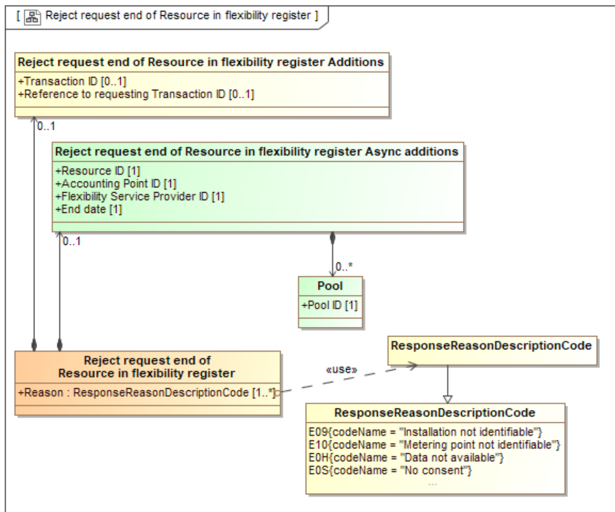
Figure 39 Class diagram: Reject request end of Resource in flexibility register
