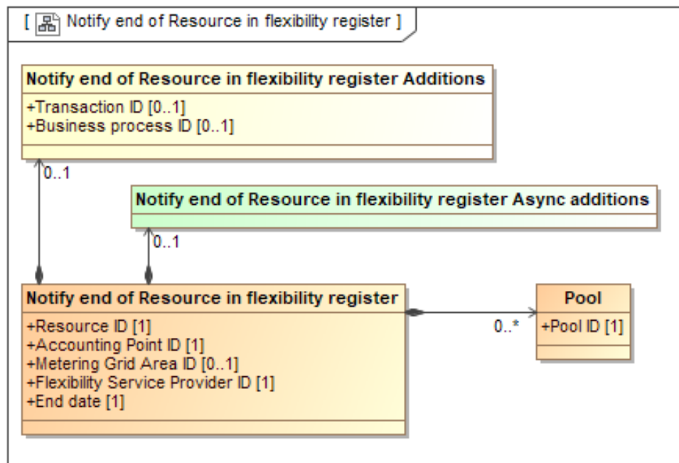
Figure 41 Class diagram: Notify end of Resource in flexibility register
