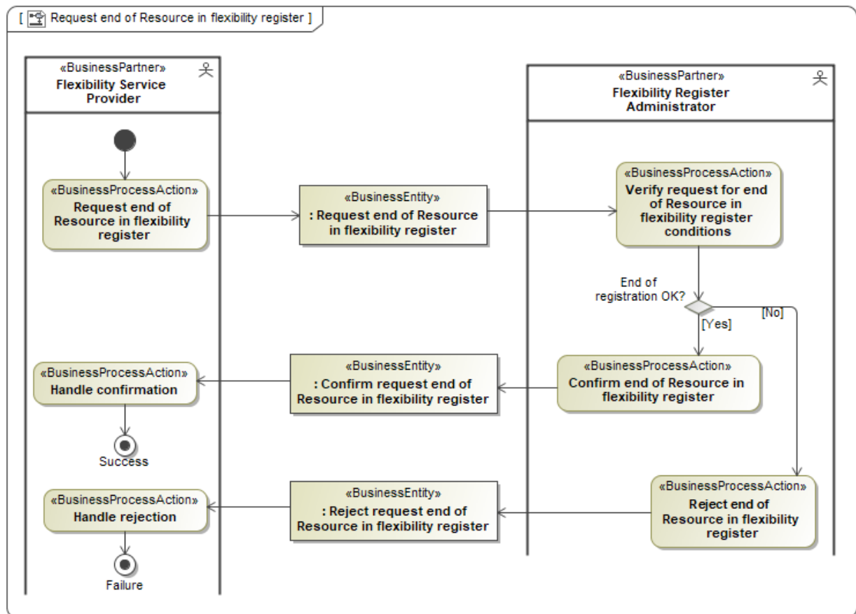
Figure 21 Business process: Request end of Resource in flexibility register
