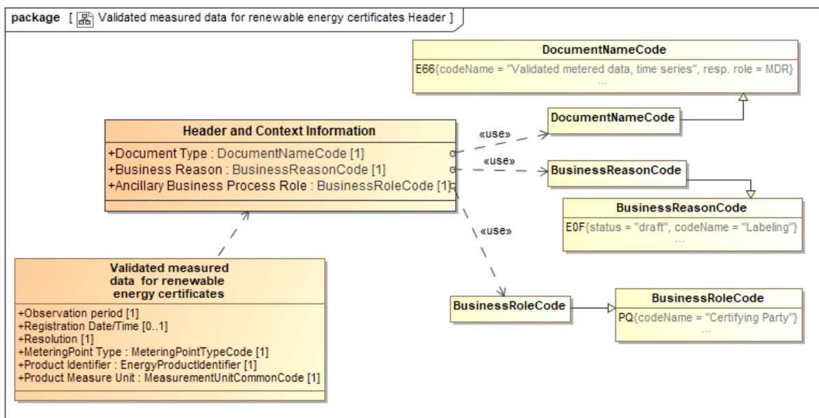
Figure 5 Header and Context Information (class diagram): Validated measured data for renewable energy certificates
