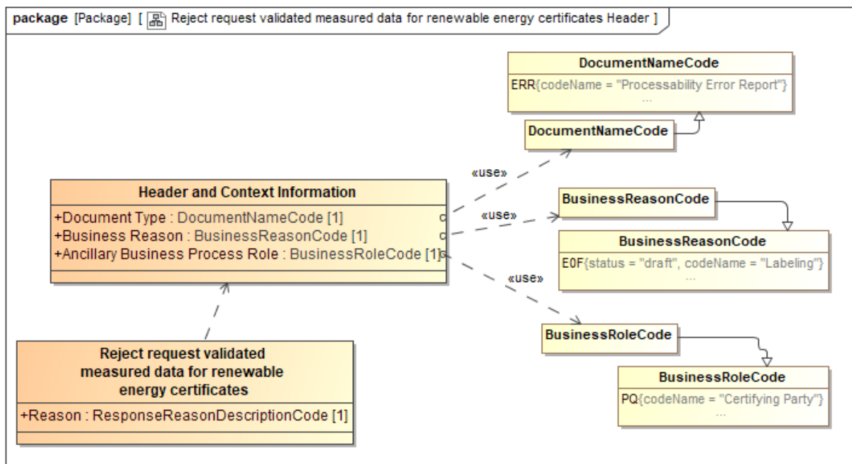
Figure 7 Header and Context Information (class diagram): Reject request validated measured data for renewable energy certificates
