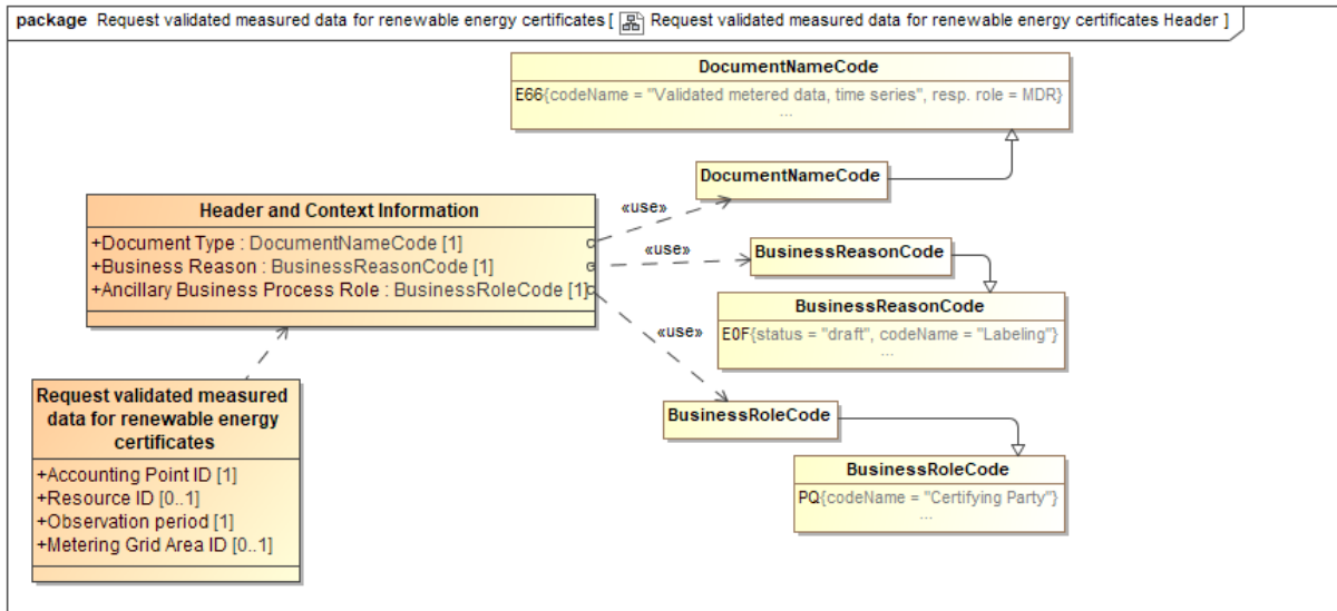
Figure 6 Header and Context Information (class diagram): Request validated measured data for renewable energy certificates
