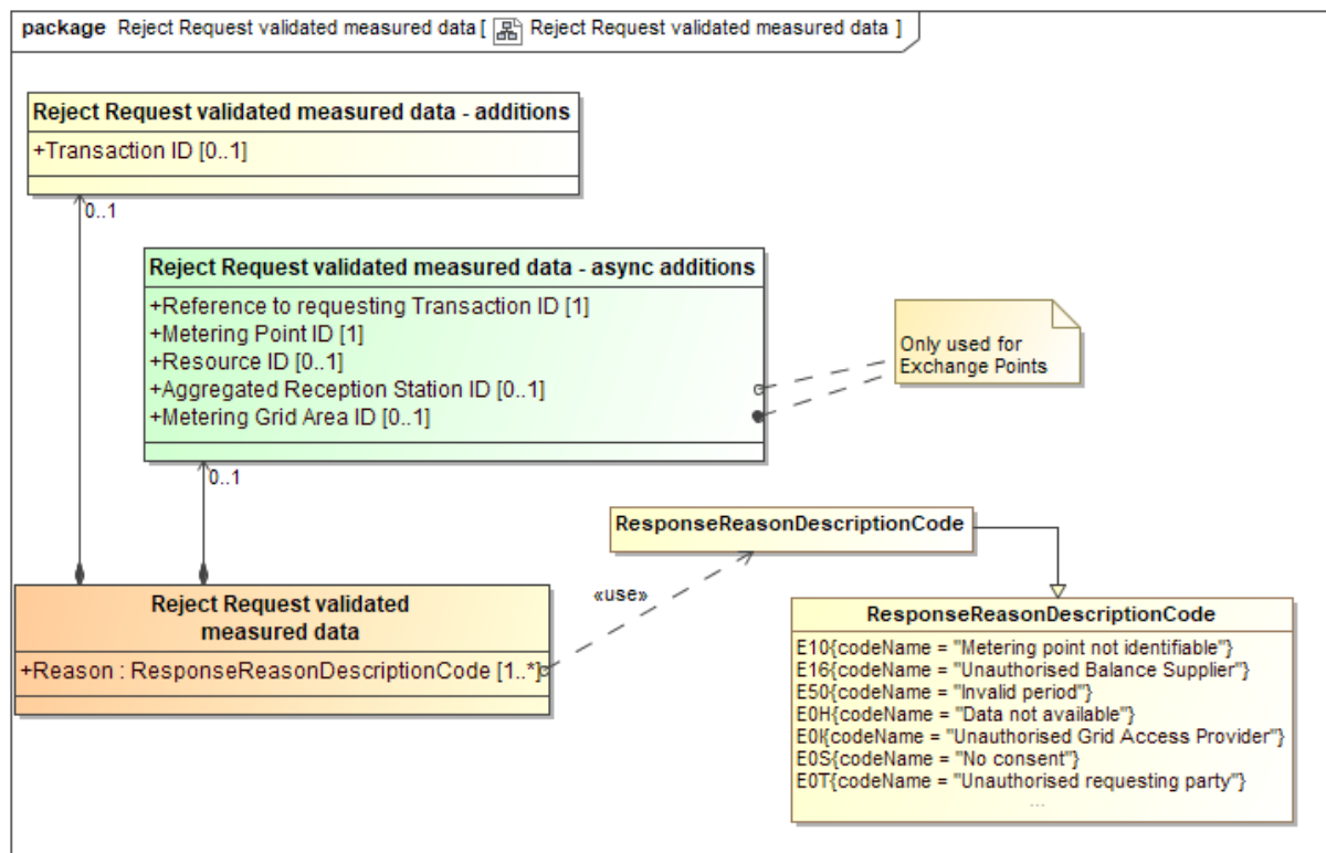
Figure 13 Class diagram: Reject Request validated measured data
