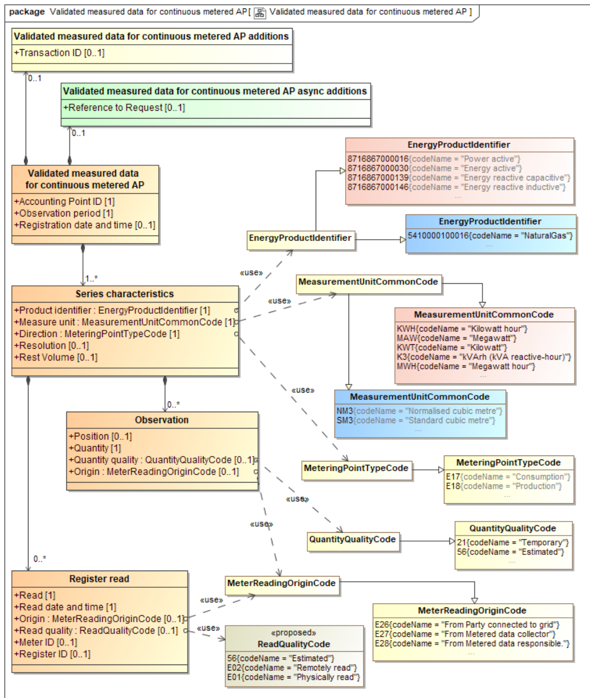
Figure 9 Class diagram: Validated measured data for continuous metered AP 5
