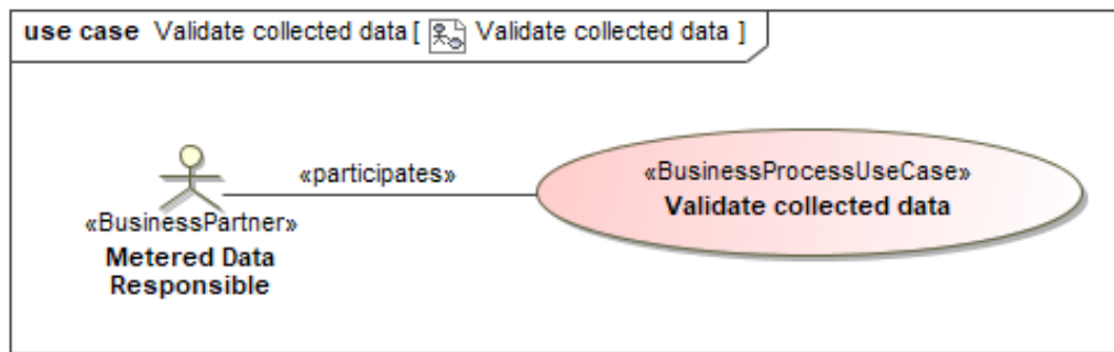
Figure 2 UseCase: Validate collected data
