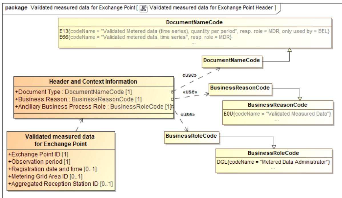
Figure 16 Class diagram: Header and Context information: Validated measured data for Exchange Points
