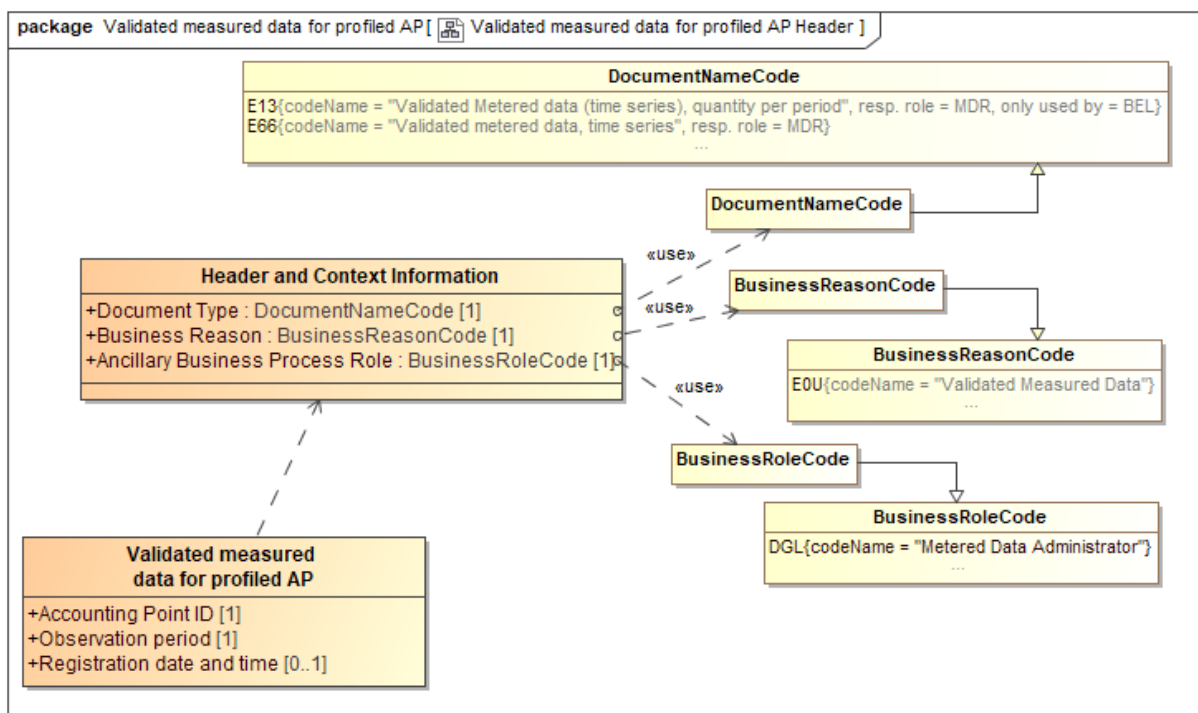
Figure 14 Class diagram: Header and Context information: Validated measured data for profiled AP
