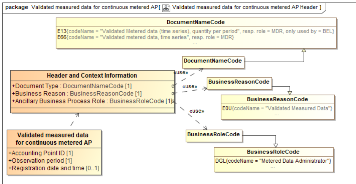
Figure 15 Class diagram: Header and Context information: Validated measured data for continuous metered AP
