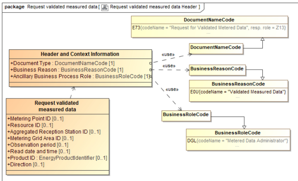
Figure 18 Class diagram: Header and Context information: Request validated measured data
