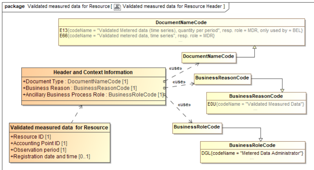
Figure 17 Class diagram: Header and Context information: Validated measured data for Resource
