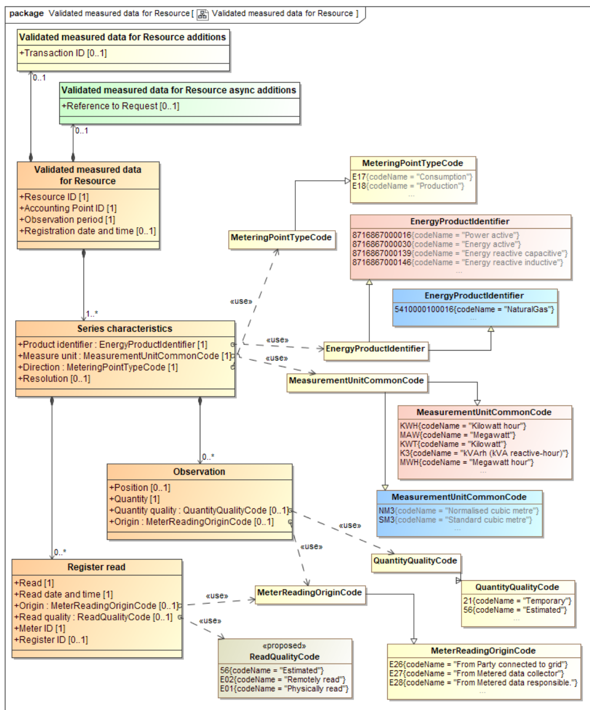
Figure 11 Class diagram: Validated measured data for Resource 12
