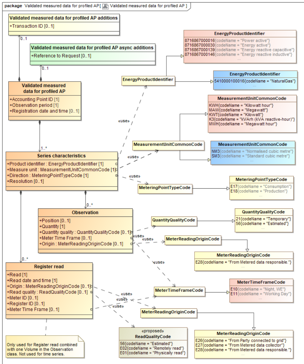
Figure 8 Class diagram: Validated measured data for profiled AP 2
