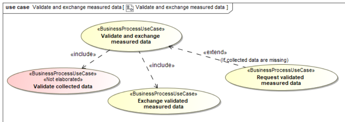
Figure 1 UseCase: Validate and exchange measured data
