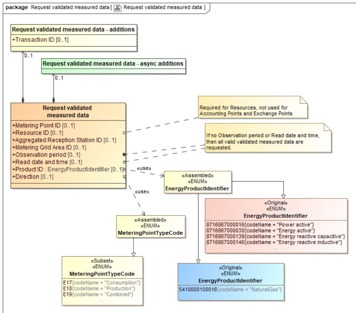
Figure 12 Class diagram: Request validated measured data
