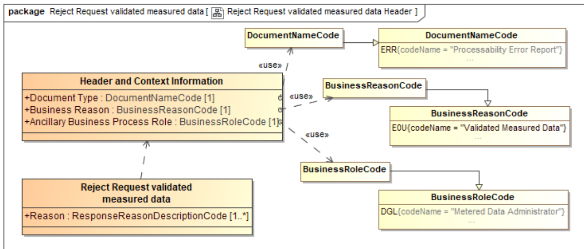
Figure 19 Class diagram: Header and Context information: Reject Request validated measured data
