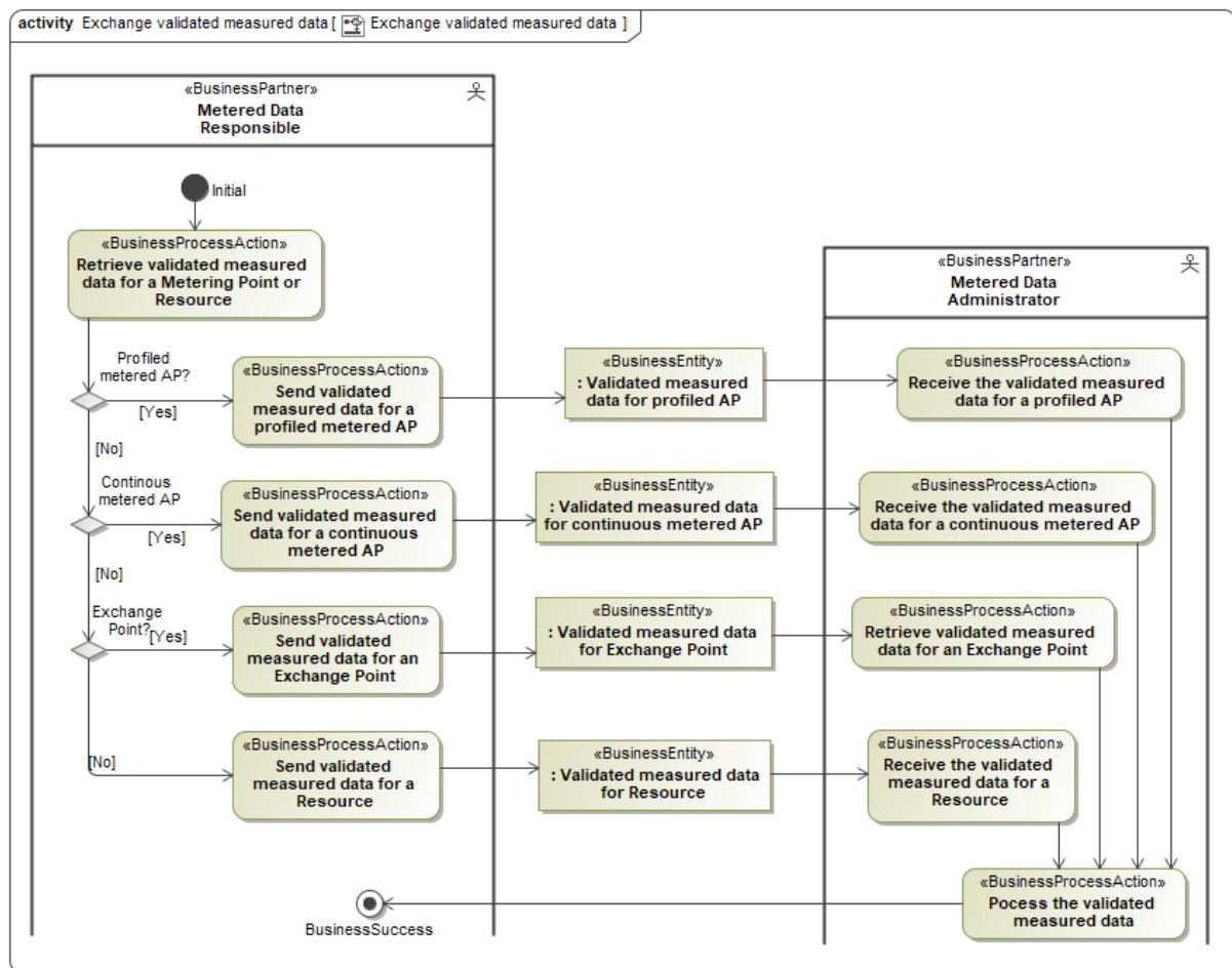
Figure 4 Business process: Exchange validated measured data
