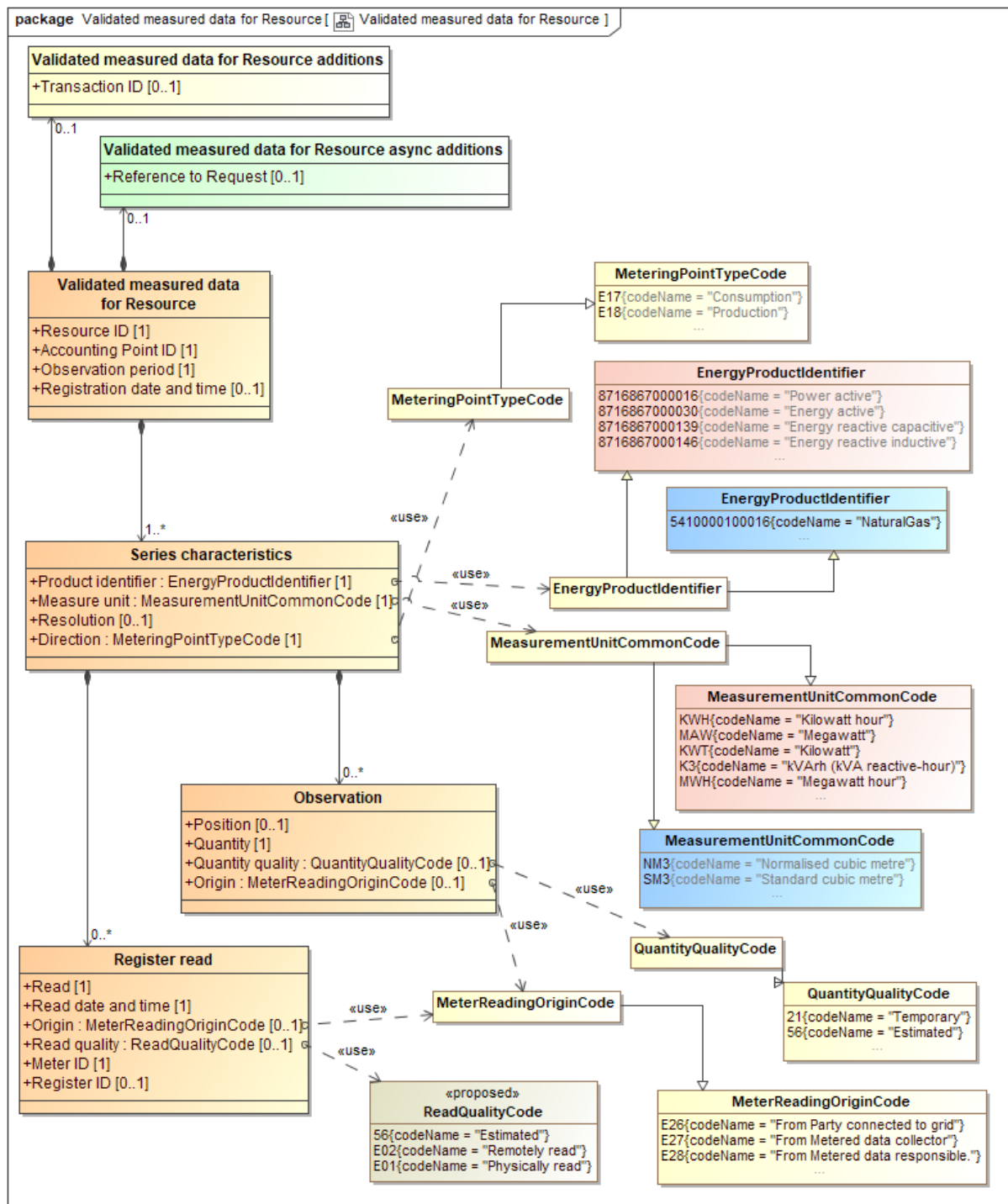
Figure 14 Class diagram: Validated measured data for Resource 13
