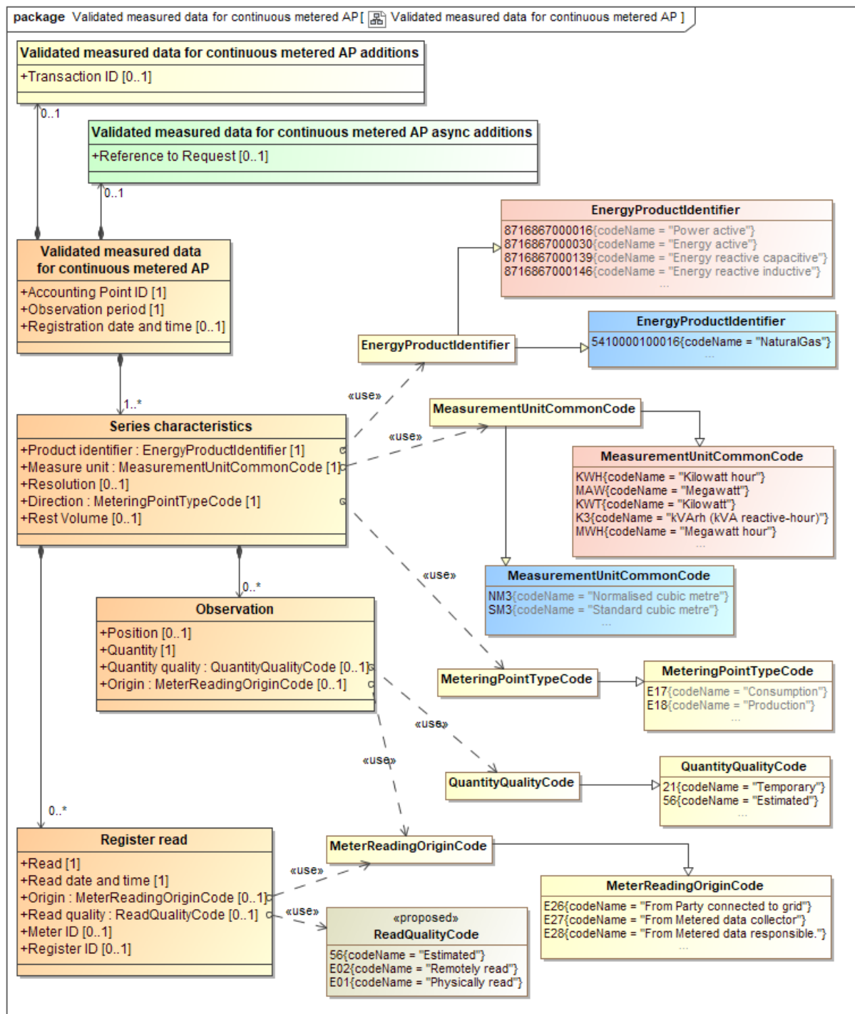
Figure 12 Class diagram: Validated measured data for continuous metered AP 6
