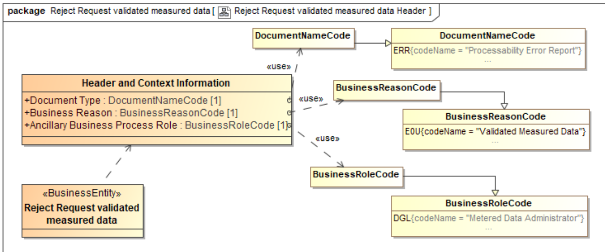
Figure 22 Class diagram: Header and Context information: Reject Request validated measured data
