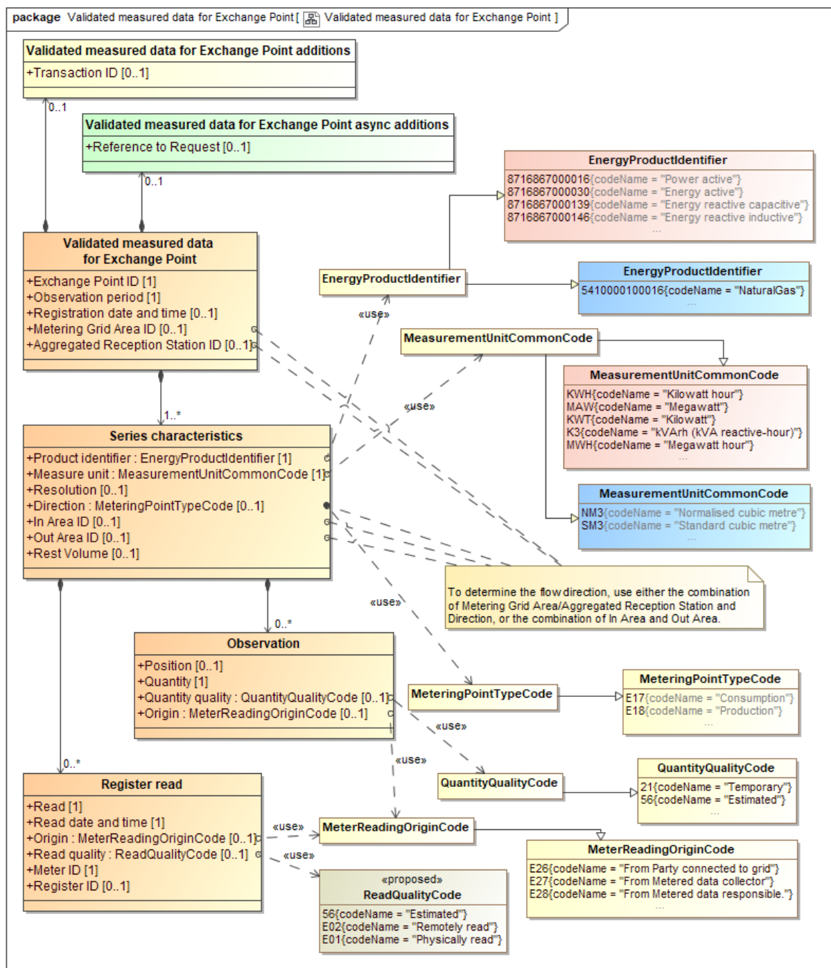
Figure 13 Class diagram: Validated measured data for Exchange Point 9
