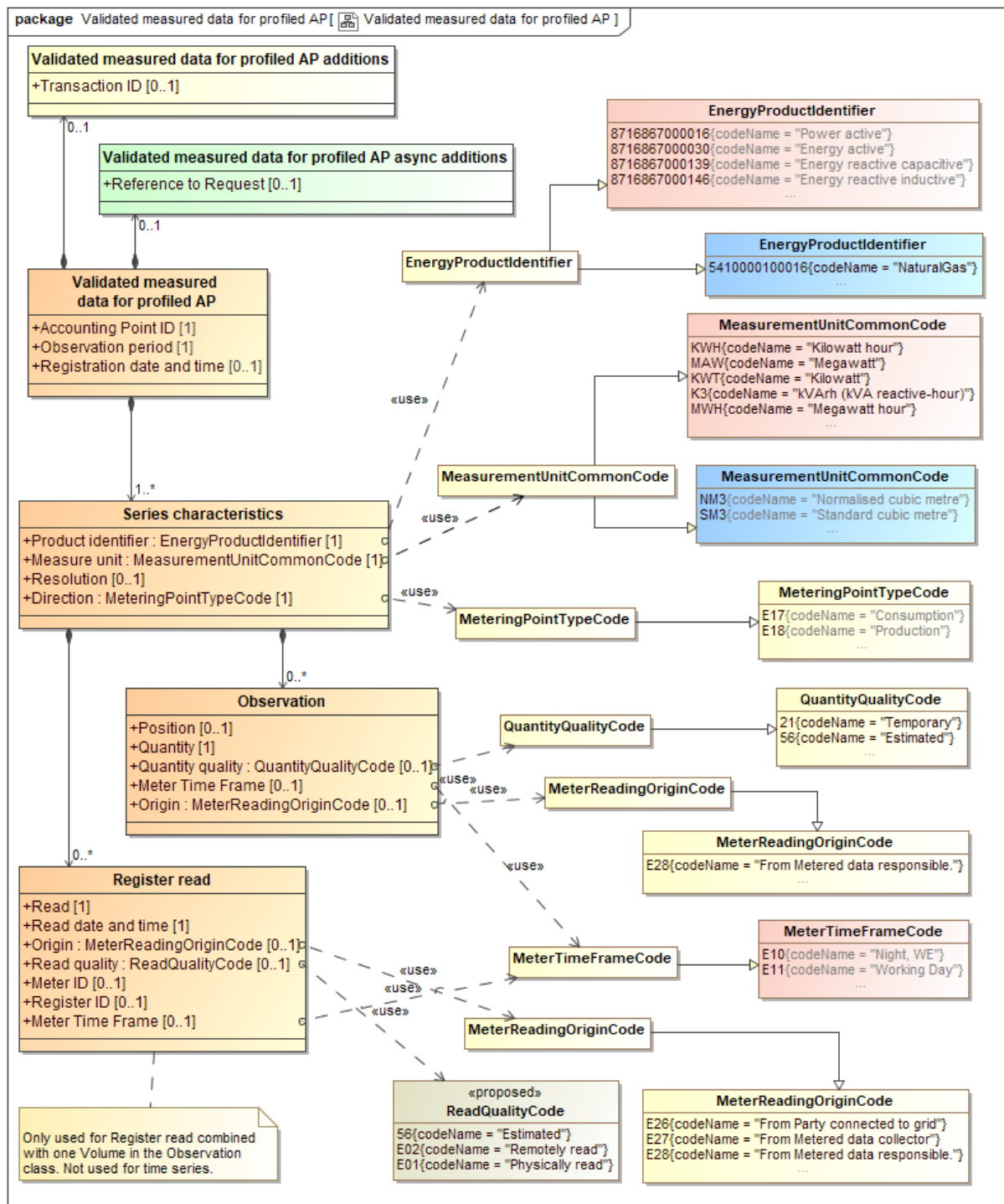
Figure 11 Class diagram: Validated measured data for profiled AP 3
