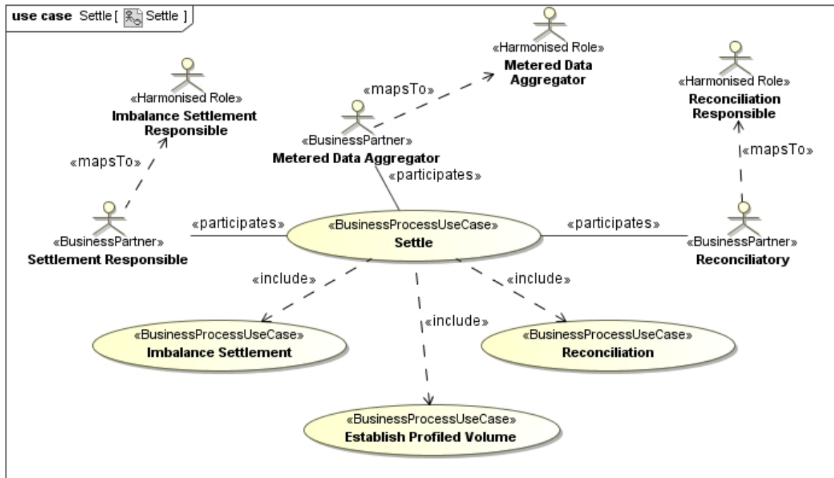
Figure 1 Settle
