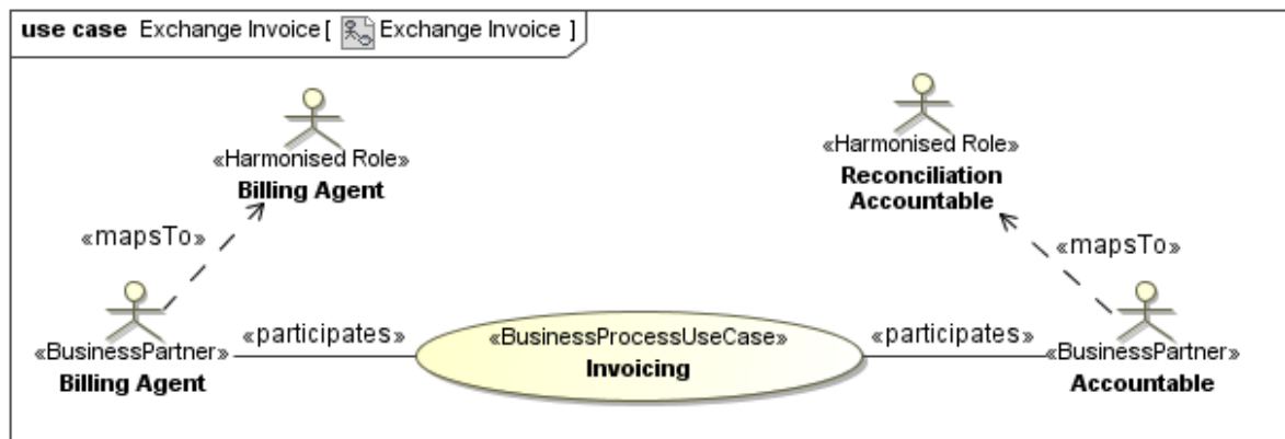
Figure 33 Invoicing
