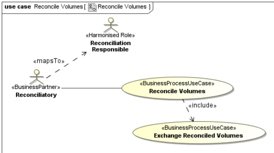
Figure 21 Reconcile Volumes
