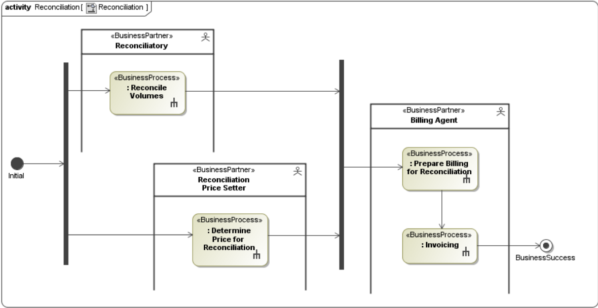
Figure 20 BP Reconciliation
