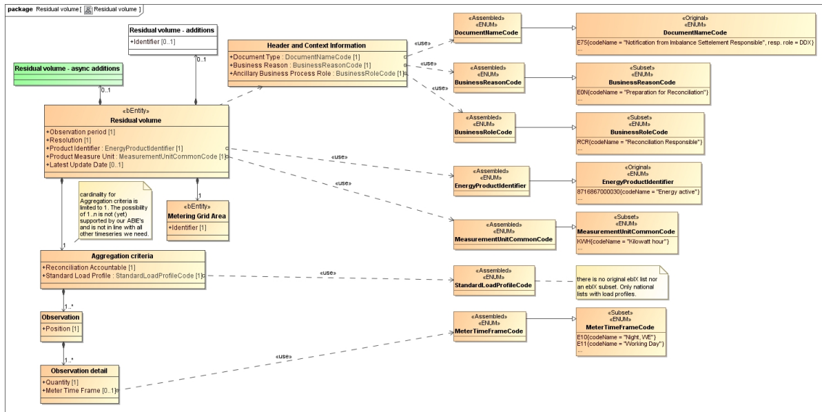
Figure 41 Residual Volume
