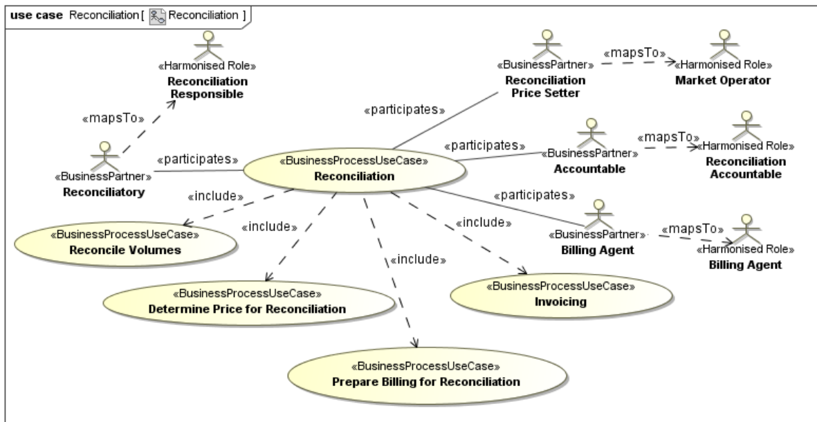
Figure 19 Reconciliation
