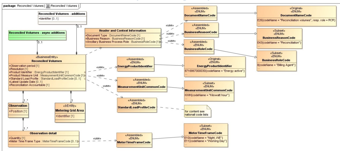
Figure 45 Reconciled Volumes
