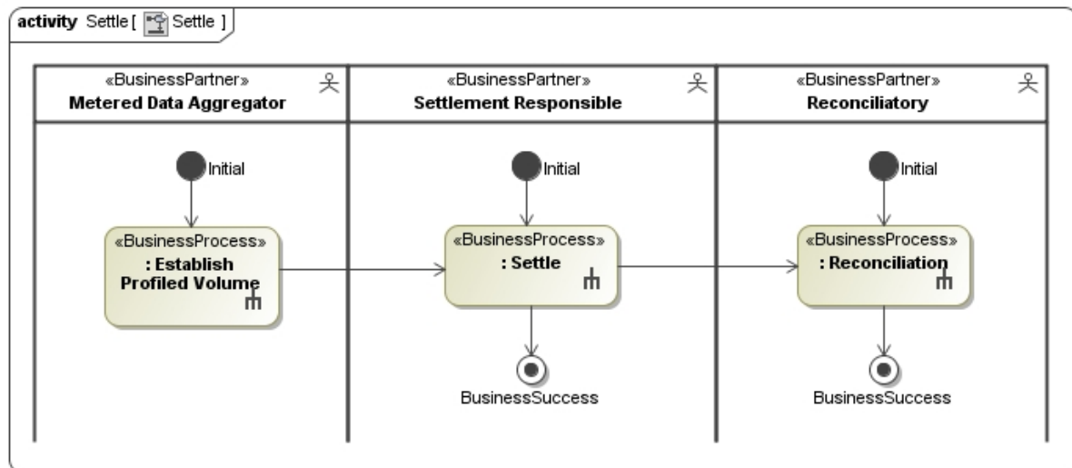
Figure 2 BP Settle
